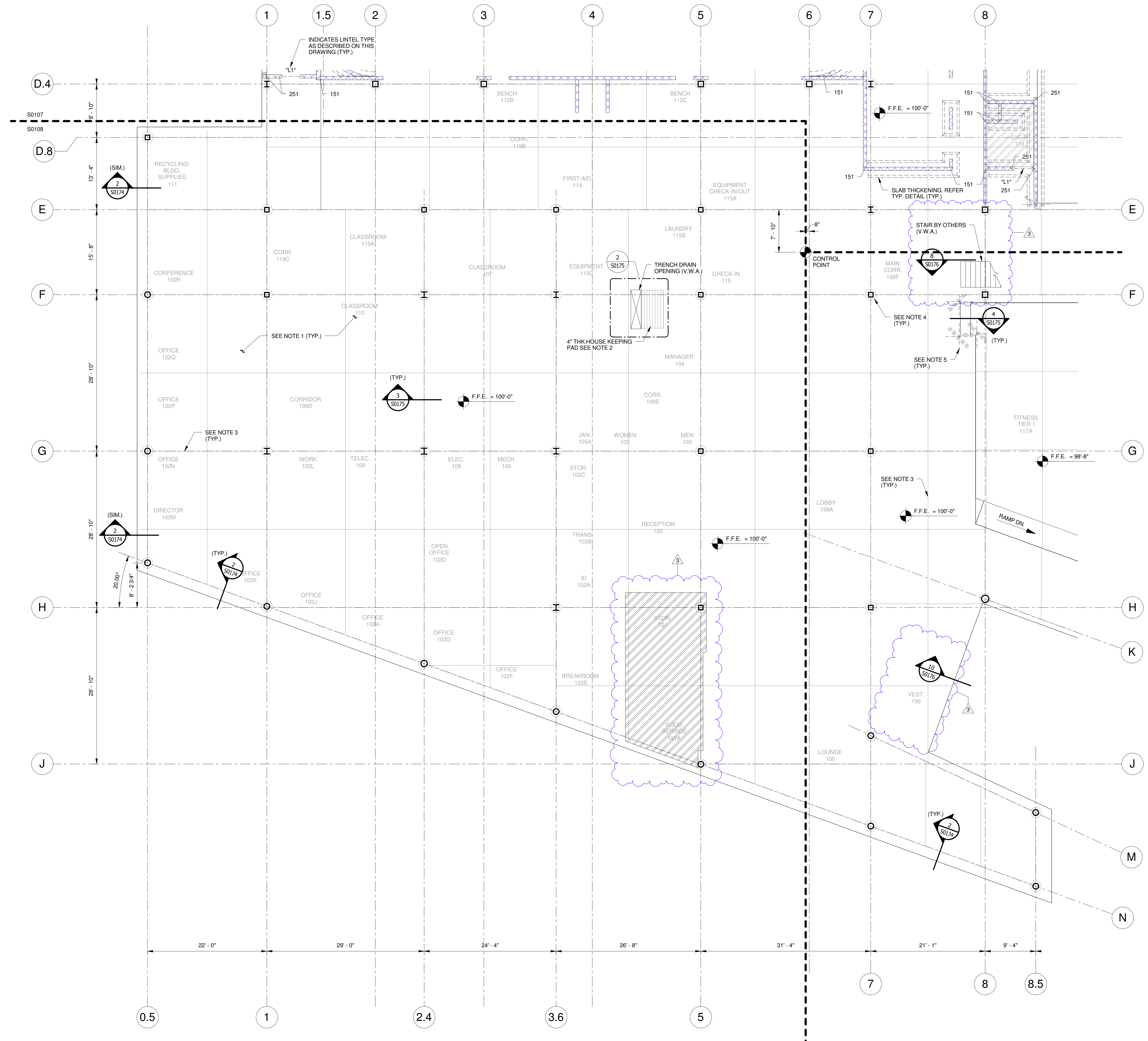
SLAB ON GRADE PLAN - AREA-C SCALE: 1/8" = 1'-0"
