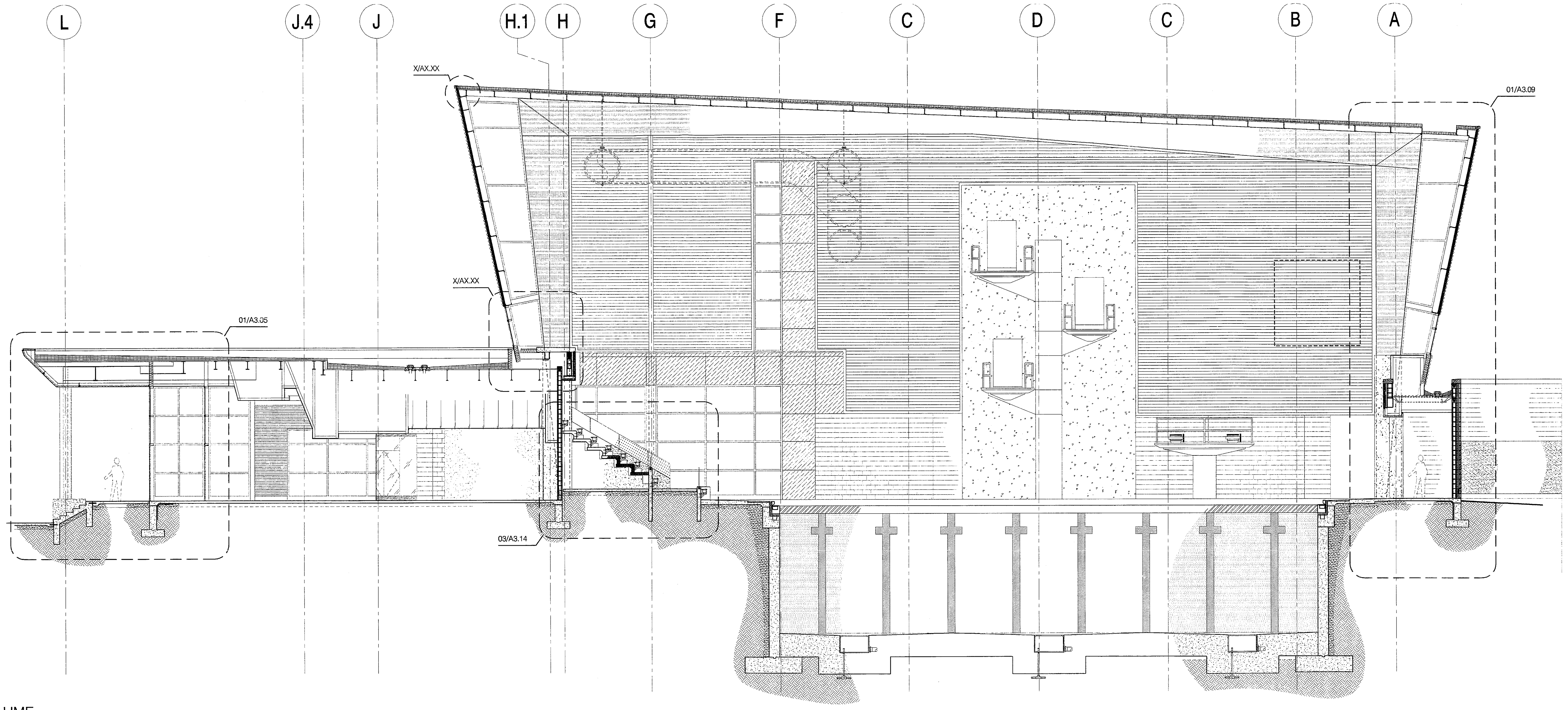
01 DIVING VOLUME BUILDING SECTION A3.01 1/8" = 1'-0"
