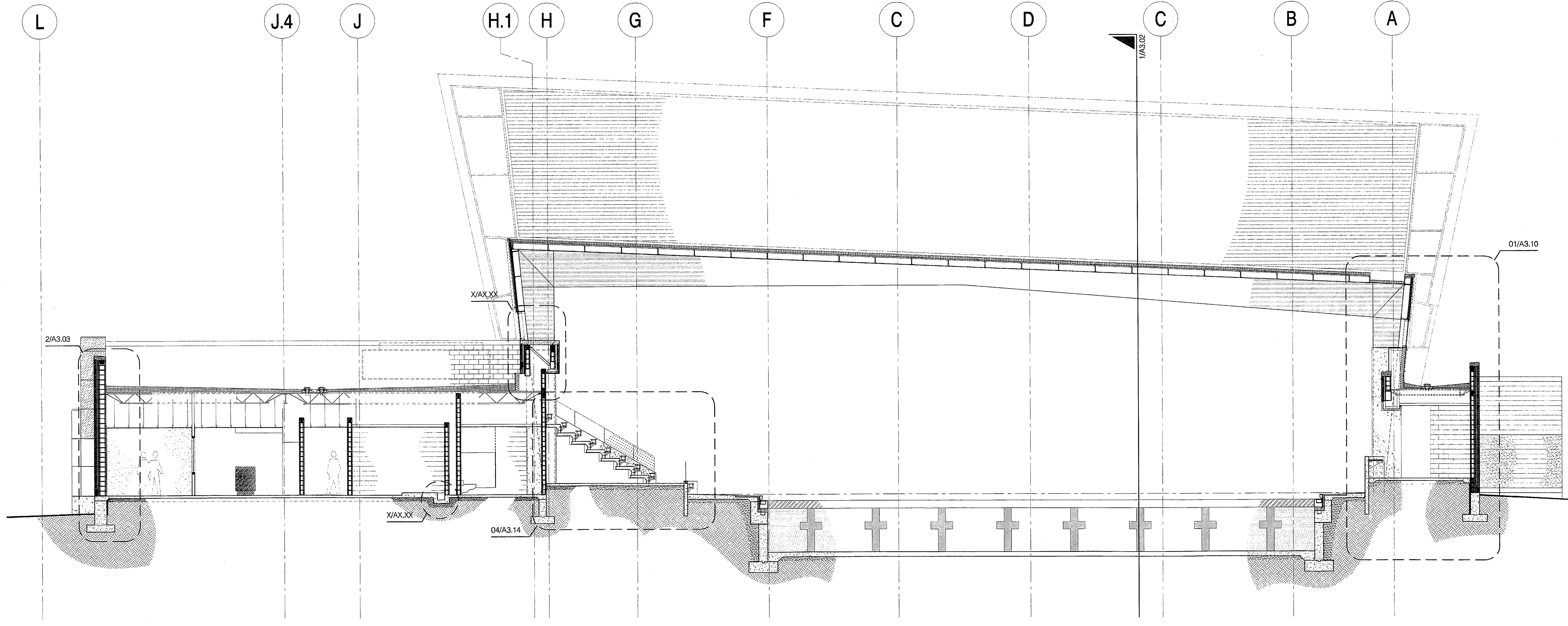
02 LOW ROOF BUILDING SECTION A3.01 1/8" = 1'-0"
