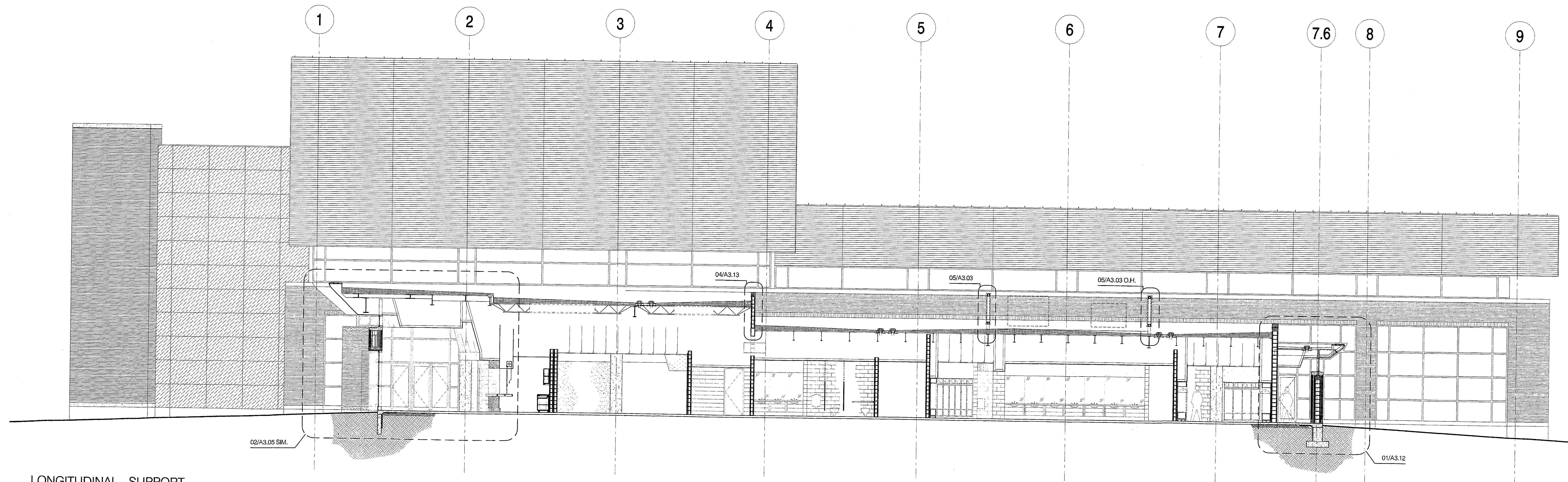
02 LONGITUDINAL - SUPPORT BUILDING SECTION
