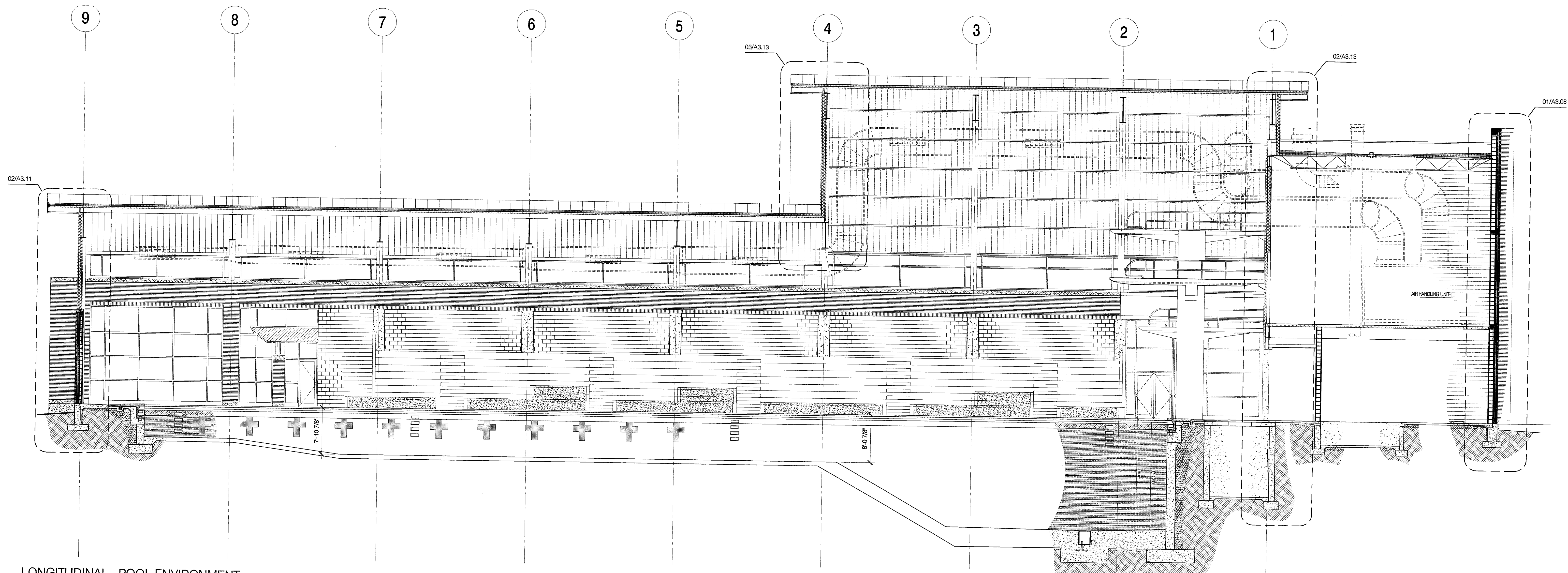
01 LONGITUDINAL - POOL ENVIRONMENT BUILDING SECTION
