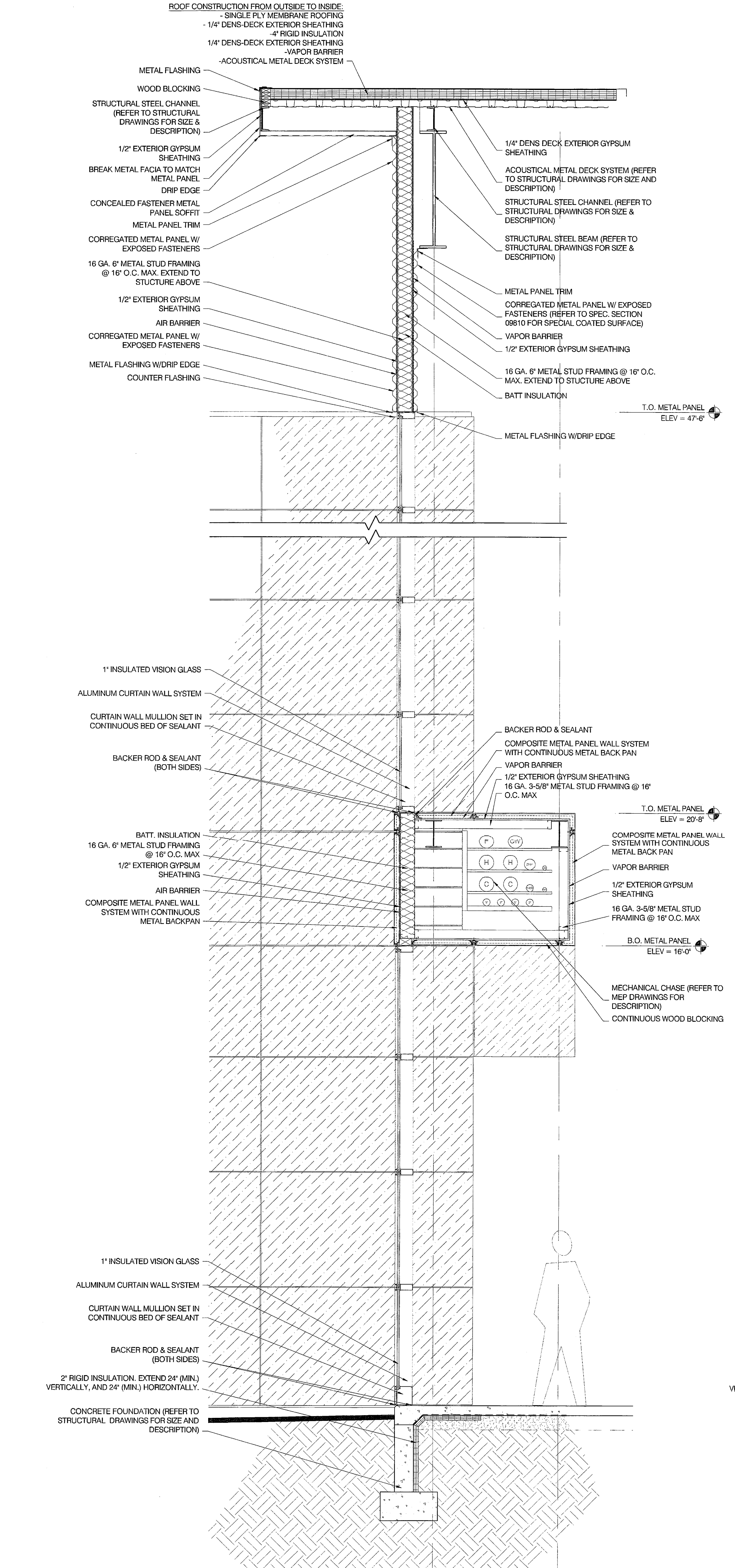
02 SOUTH CURTAINWALL WALL SECTION A3.07 1/2" = 1'-0"
