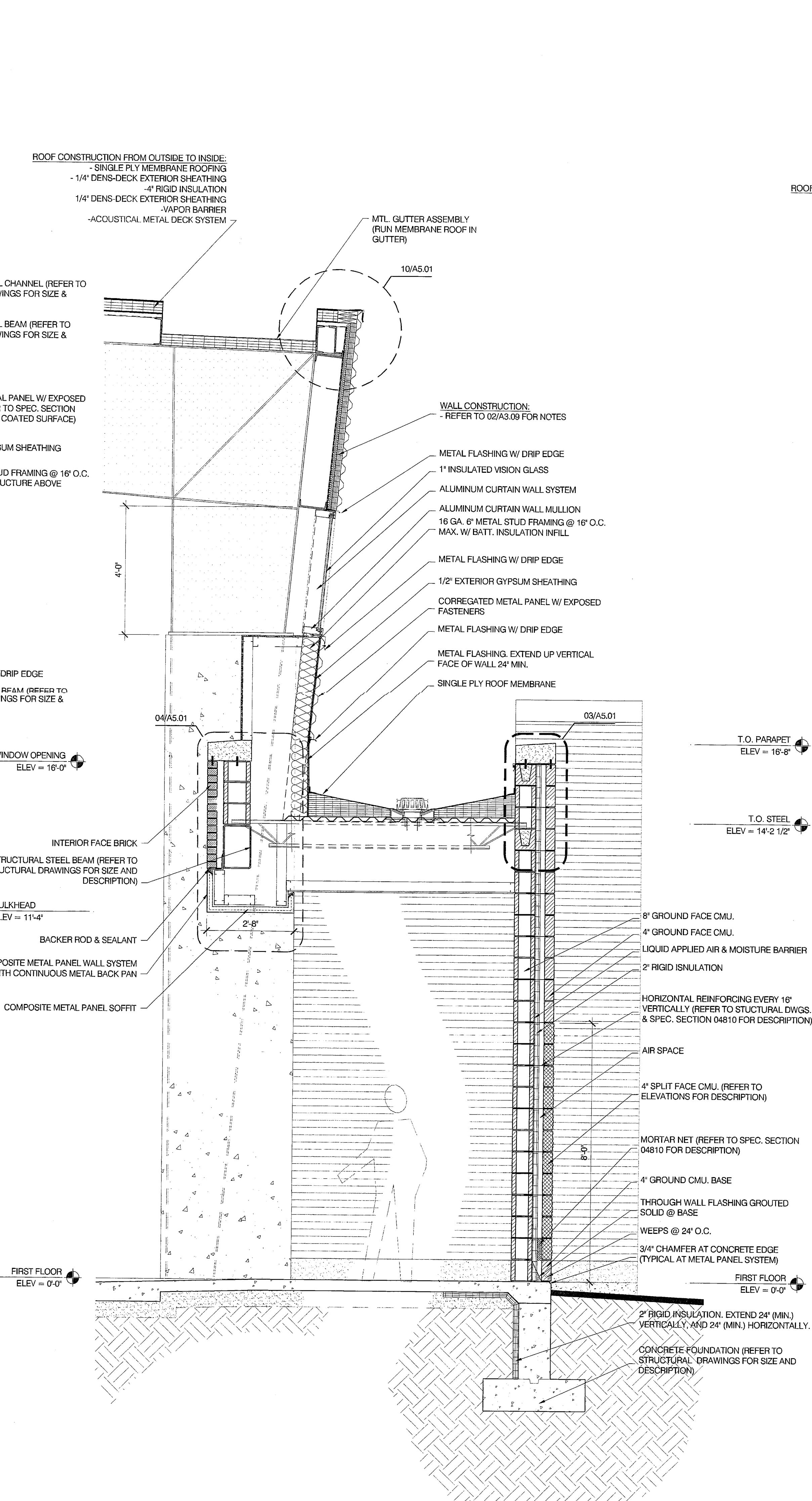
02 WALL SECTION A3.10 1/2" = 1'-0"
