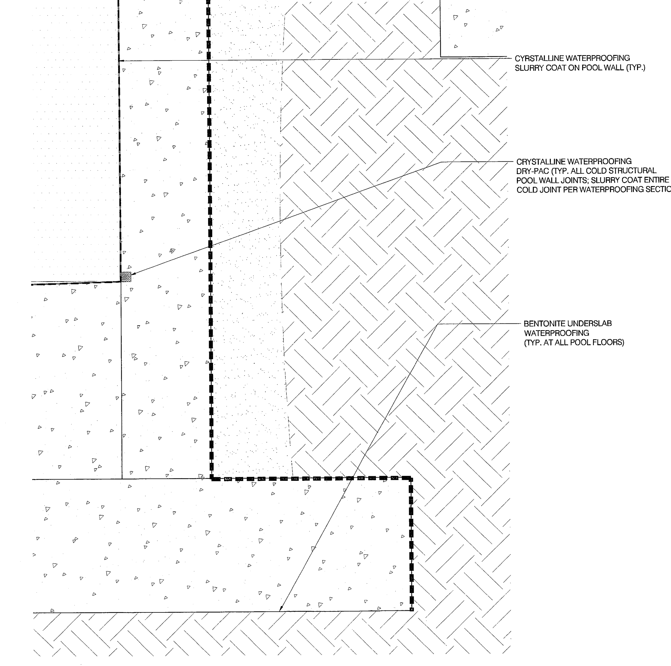
01 POOL WALL - DIVING END WALL SECTION A8.02 1" = 1'-0"
