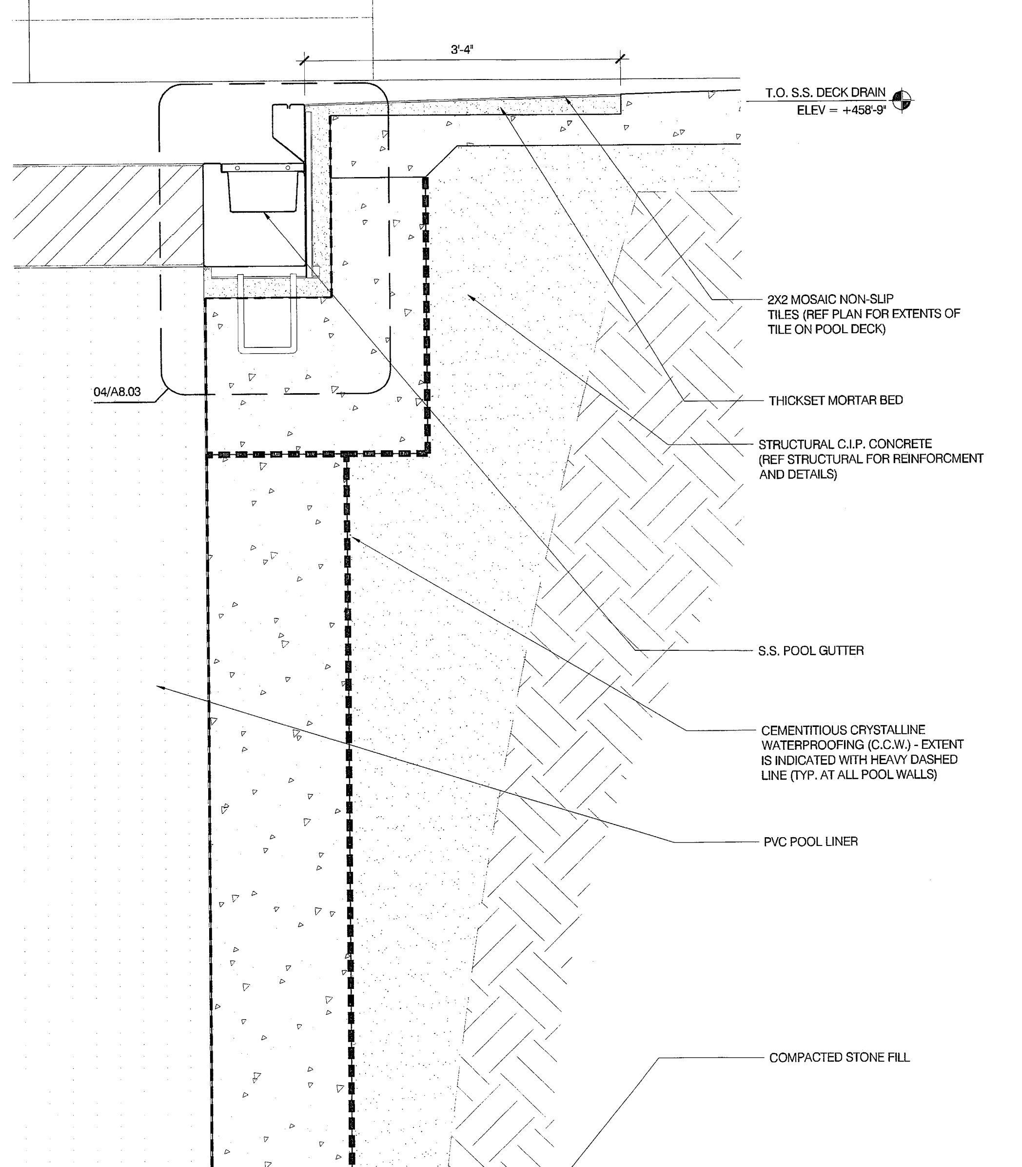
02 POOL WALL - DIVING END WALL SECTION A8.02 1" = 1'-0"
