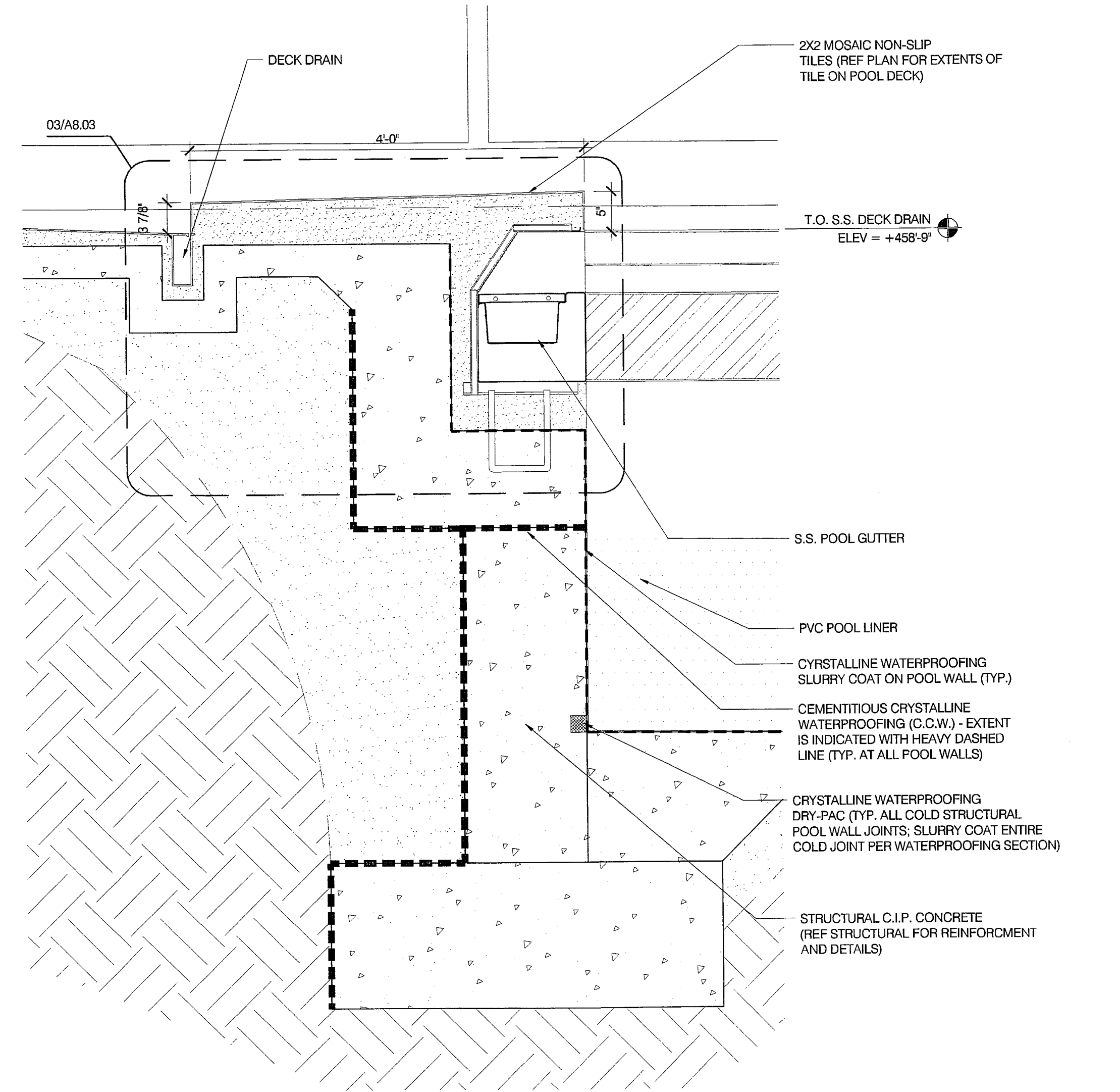
03 POOL WALL - SHALLOW END WALL SECTION A8.02 1" = 1'-0"
