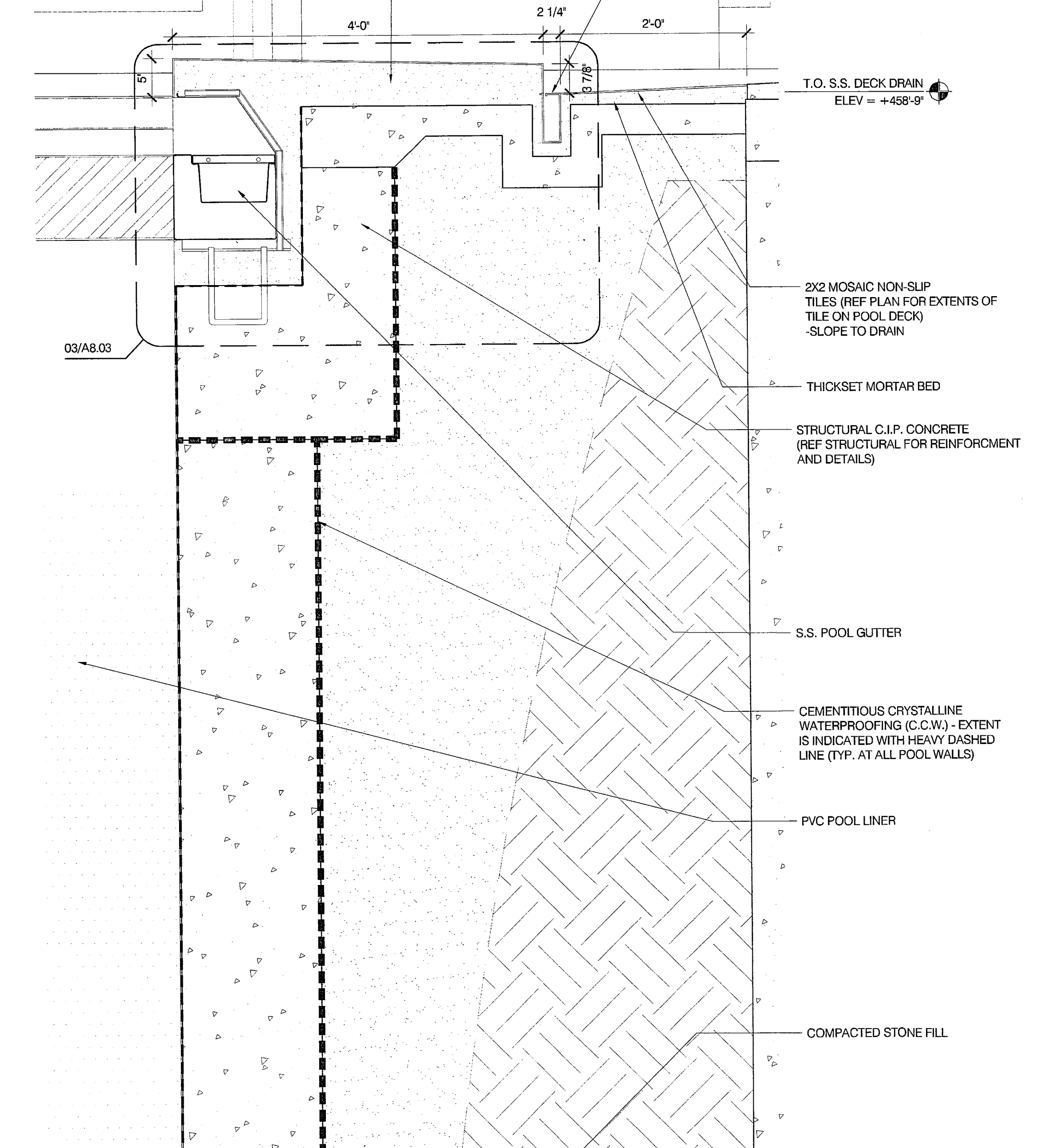
01 POOL WALL - DIVING END WALL SECTION A8.02 1" = 1'-0"
