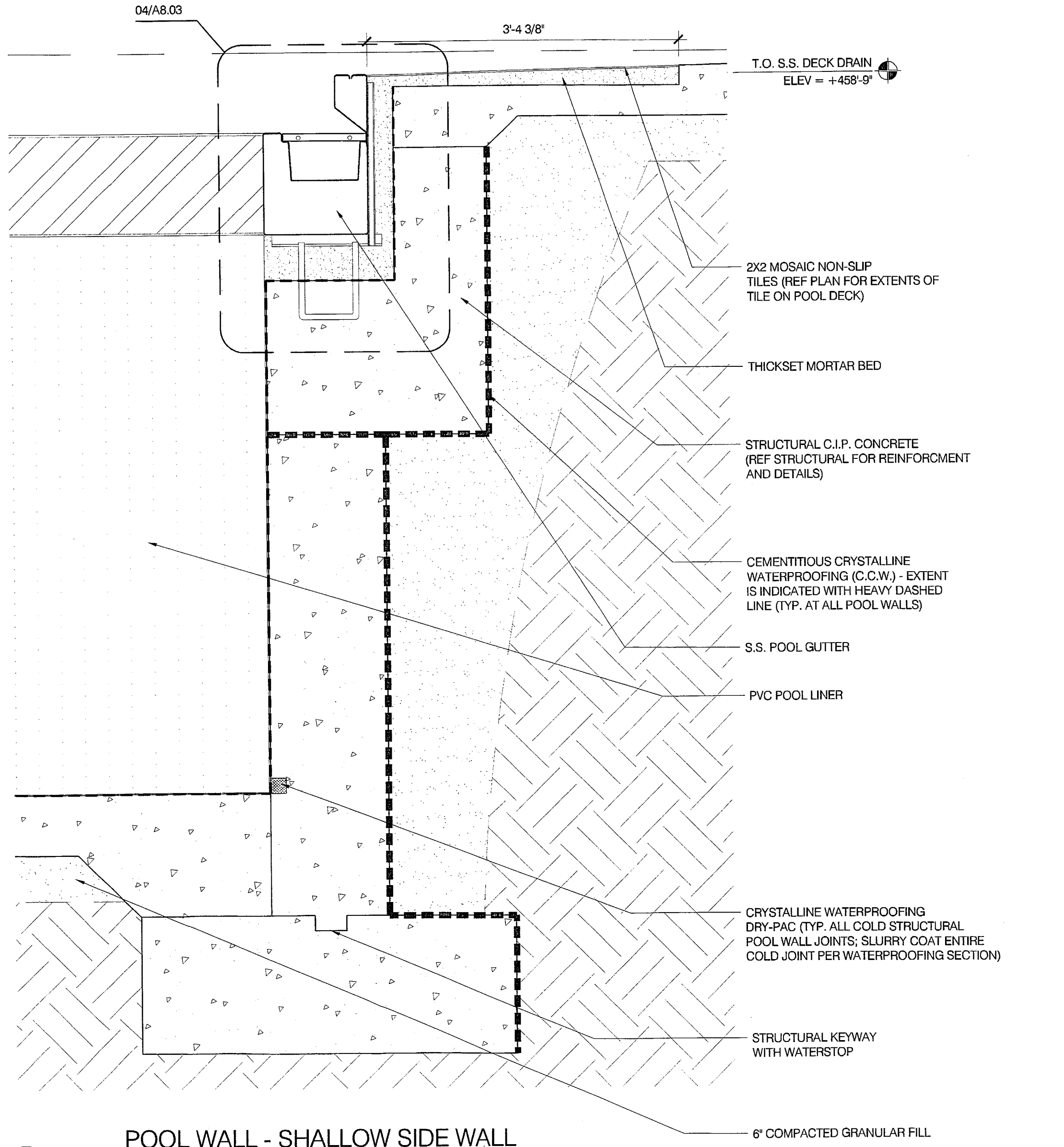
04 POOL WALL - SHALLOW SIDE WALL SECTION A8.02 1" = 1'-0"
