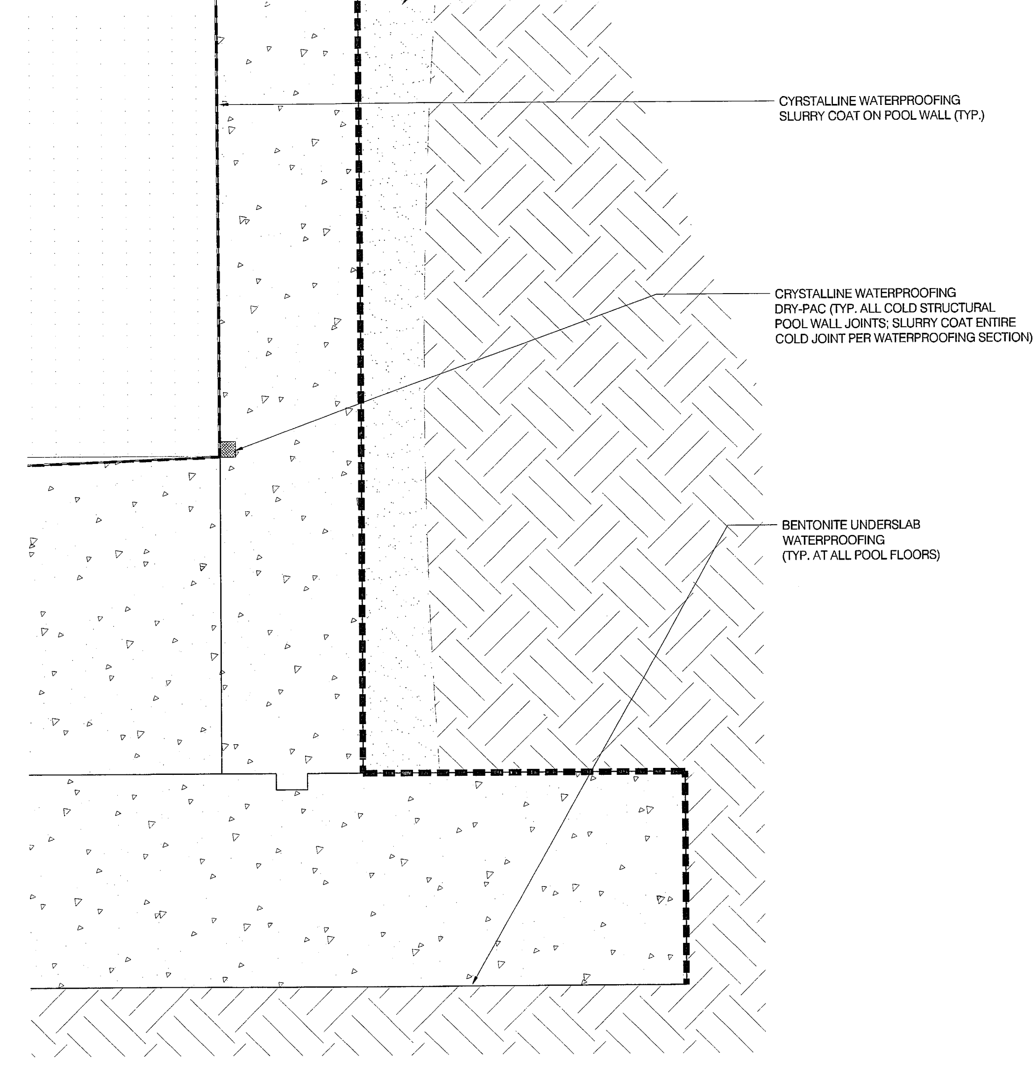
02 POOL WALL - DIVING END WALL SECTION A8.02 1" = 1'-0"
