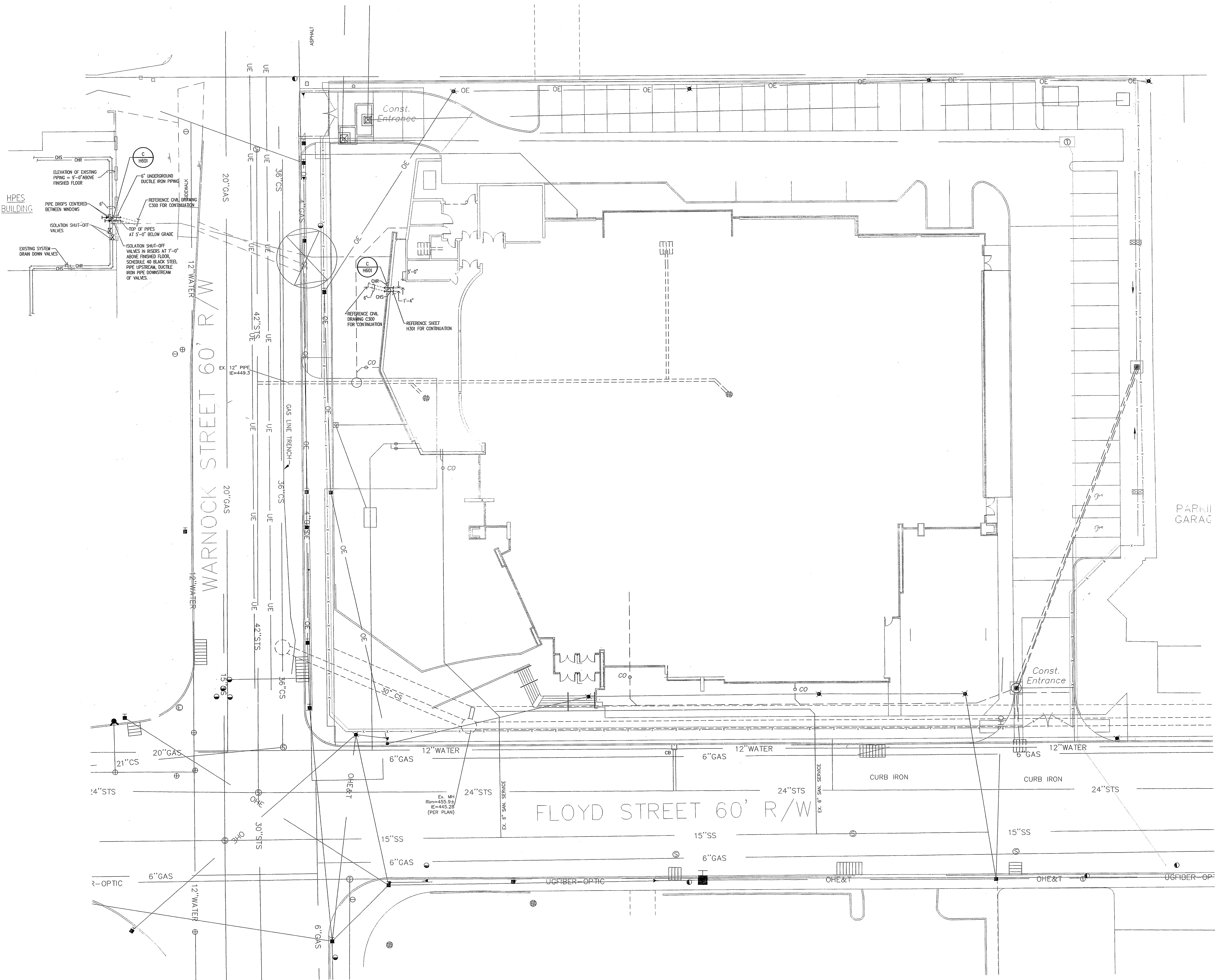
SITE PLAN - HVAC SCALE: 1/16" = 1'-0"
