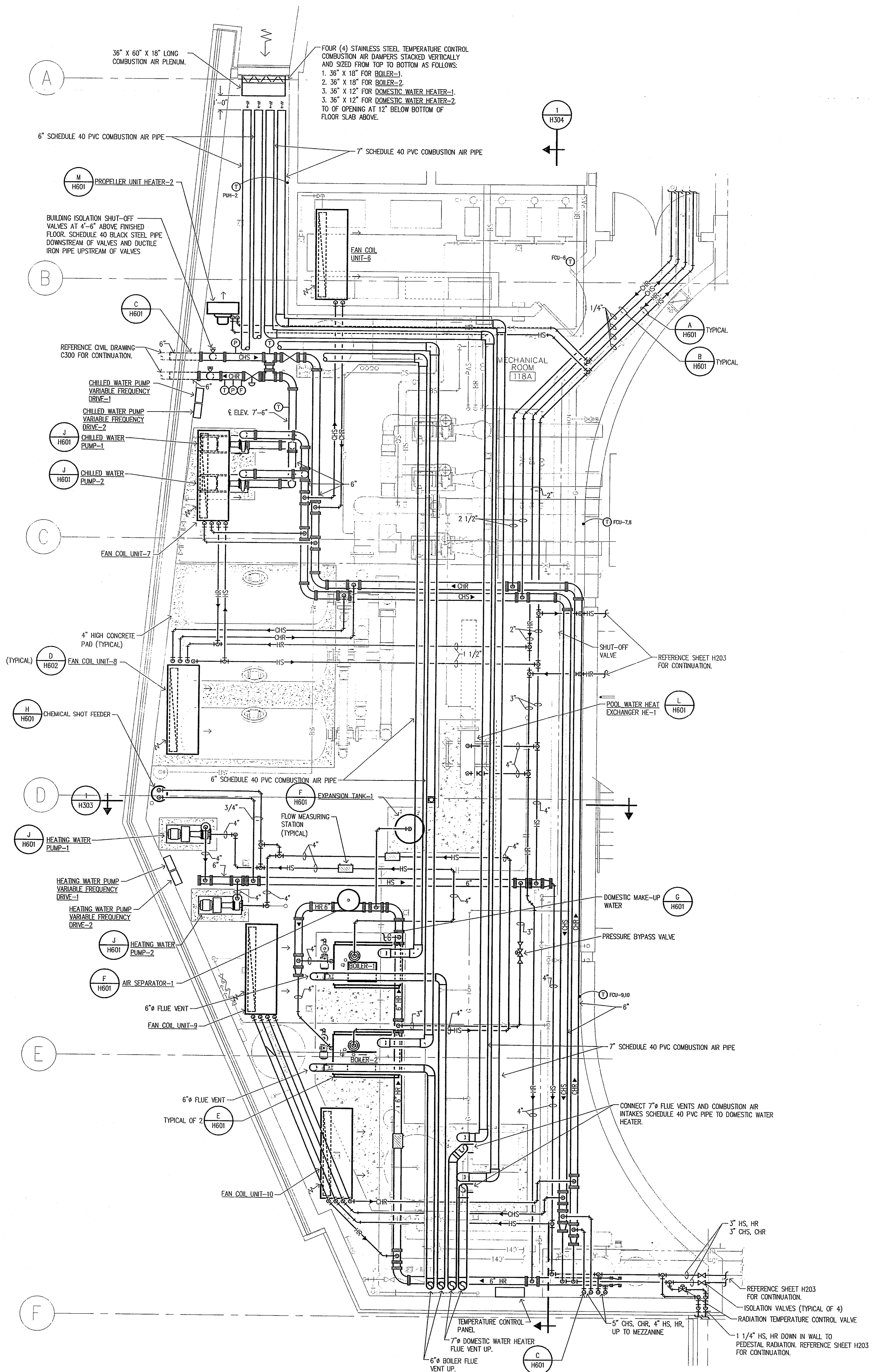
ENLARGED MAIN LEVEL MECHANICAL ROOM 118A PLAN - HVAC SCALE: 1/4" = 1'-0"
