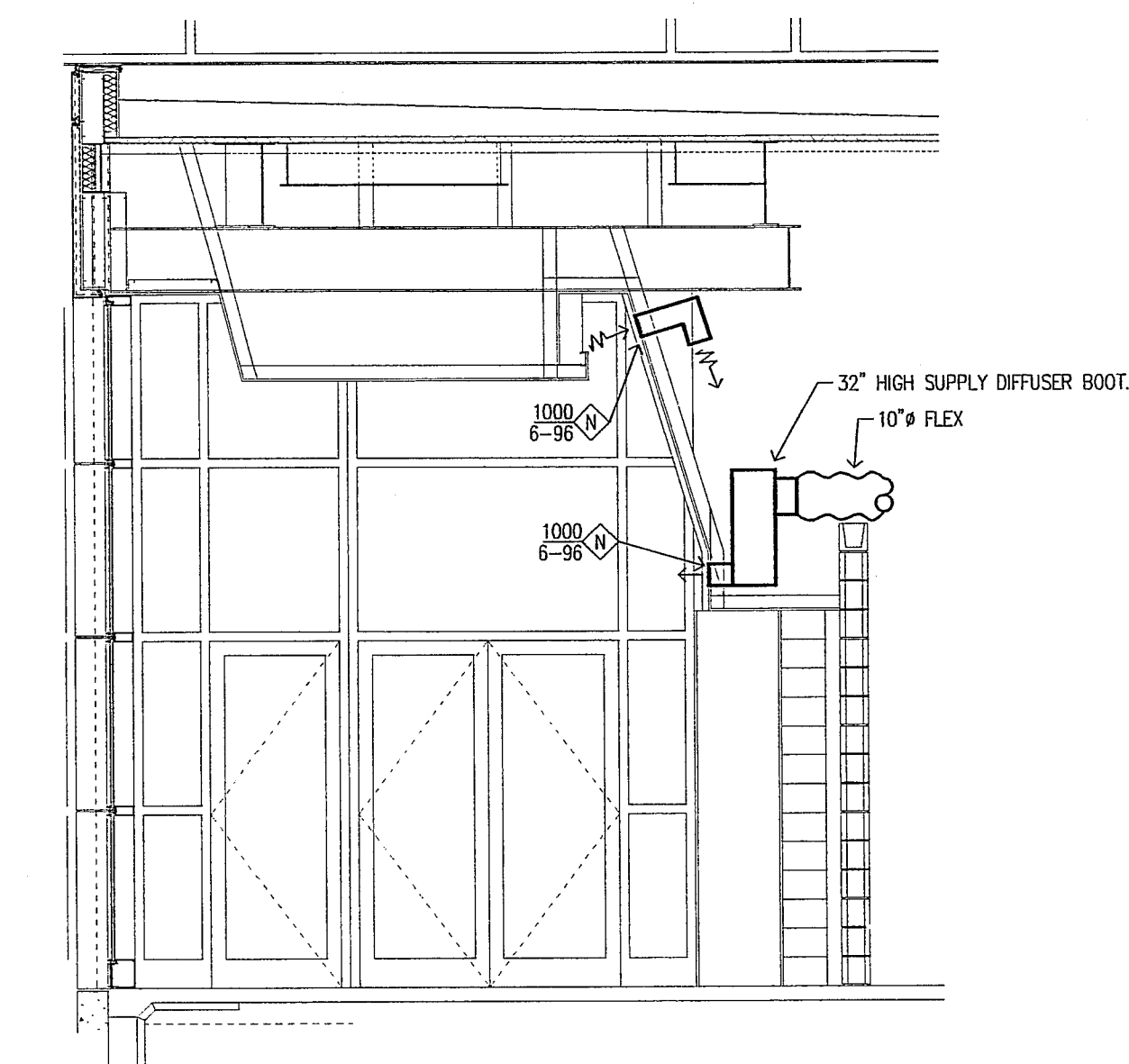
SECTION 3 SCALE 1/4" = 1'-0"
