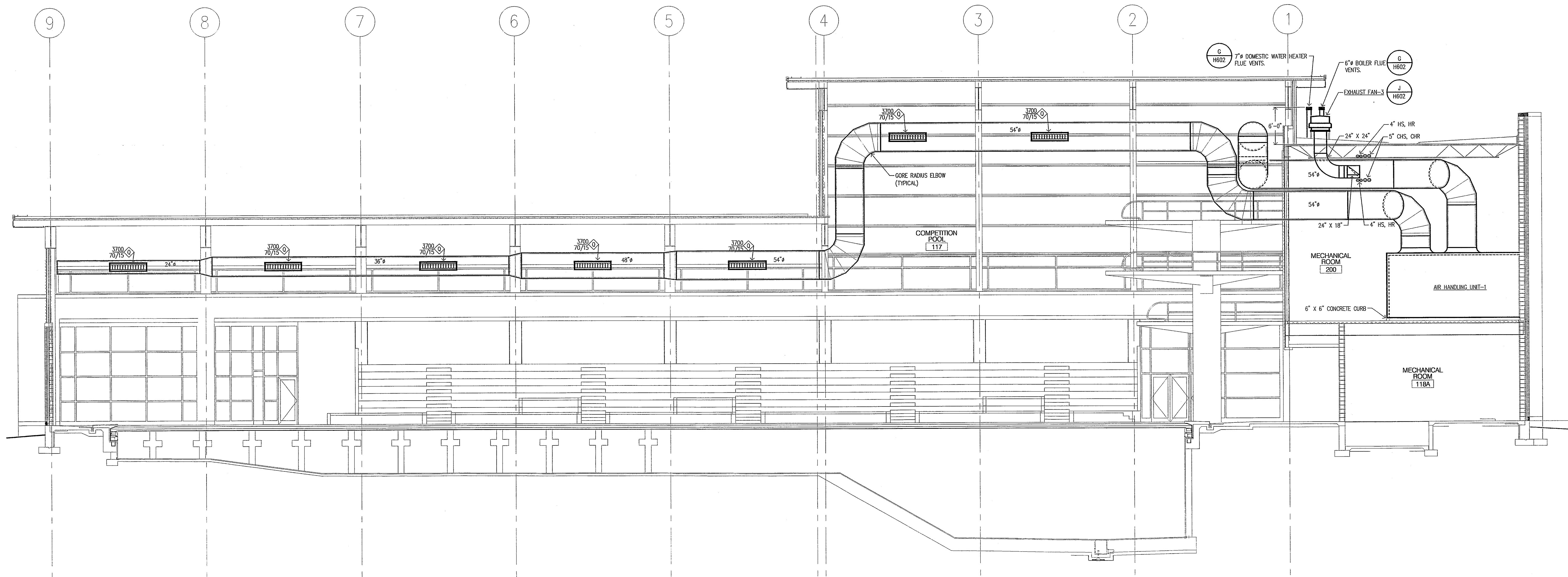
SECTION 1 SCALE 1/8" = 1'-0"
