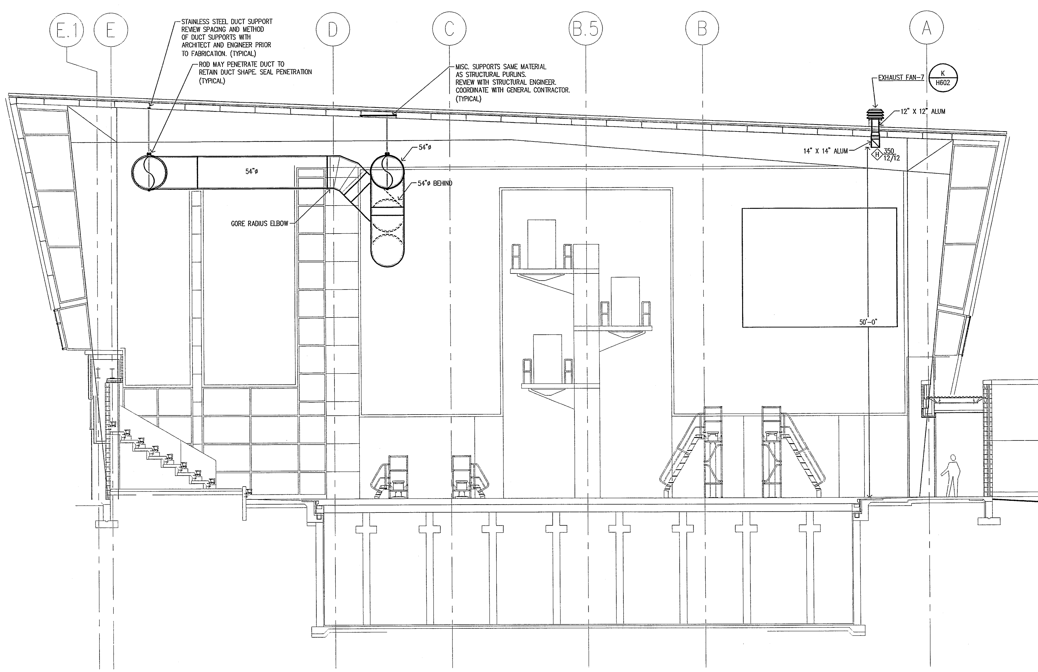
SECTION 2 SCALE 1/8" = 1'-0"
