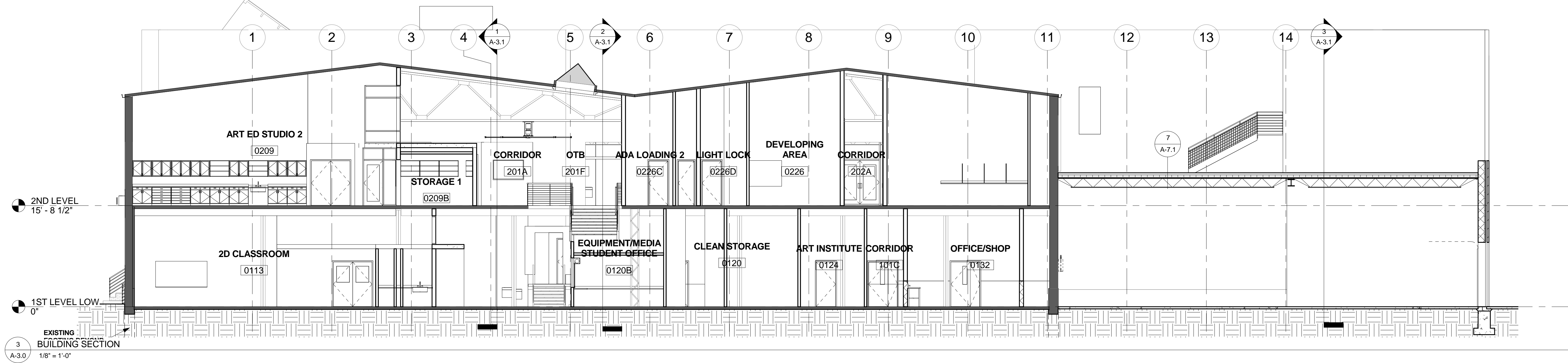
2 BUILDING SECTION 1/8" = 1'-0"
