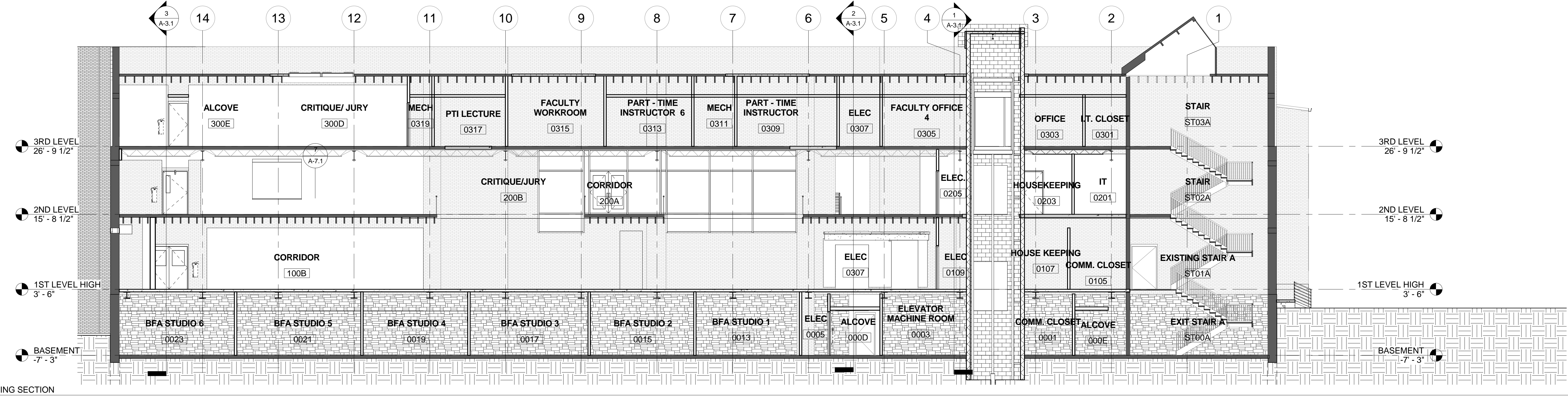
4 BUILDING SECTION 1/8" = 1'-0"
