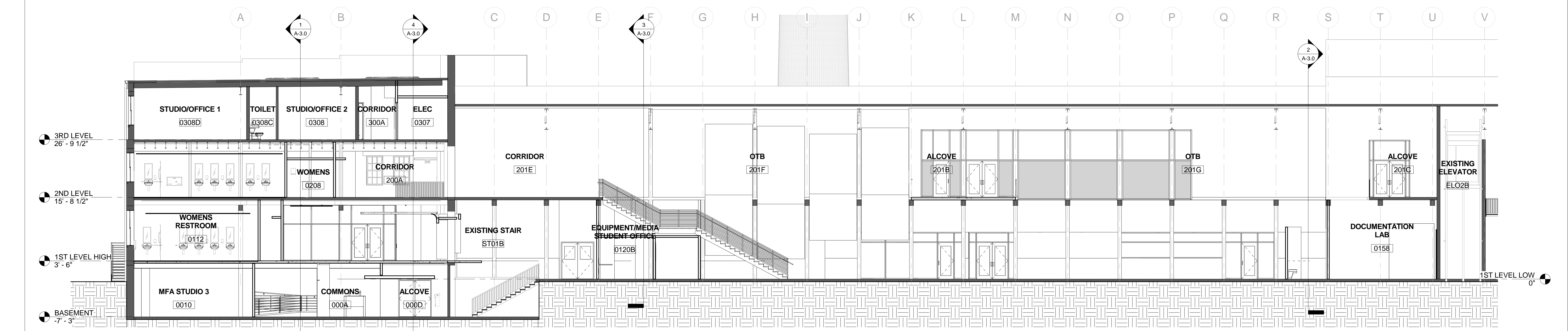
2 BUILDING SECTION A-3.1 1/8" = 1'-0"
