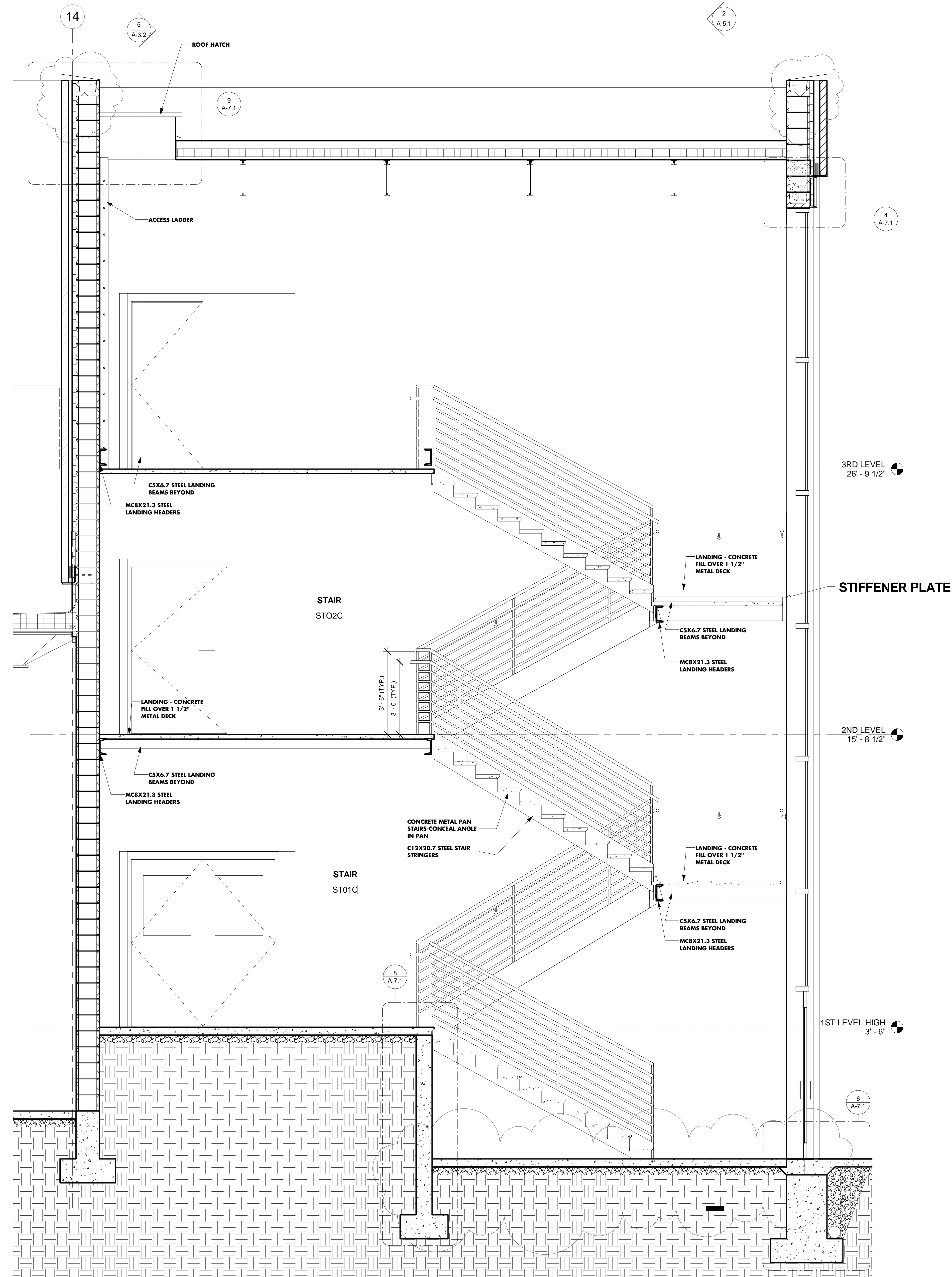
1 ENLARGED SECTION- STAIR A-5.1 1/2" = 1'-0"
