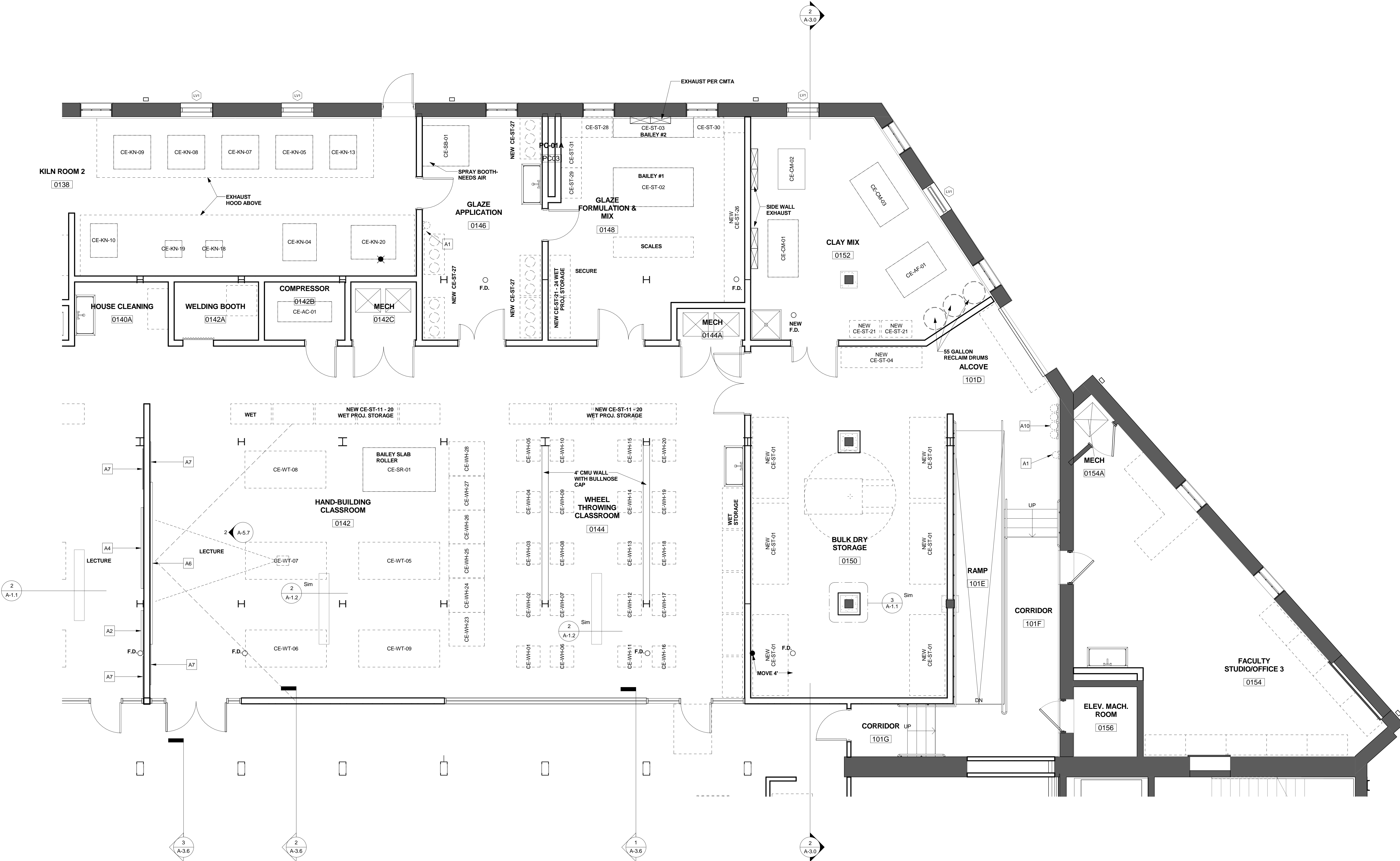
1 ENLARGED PLAN - CERAMICS 2 A-5.23 1/4" = 1'-0"
