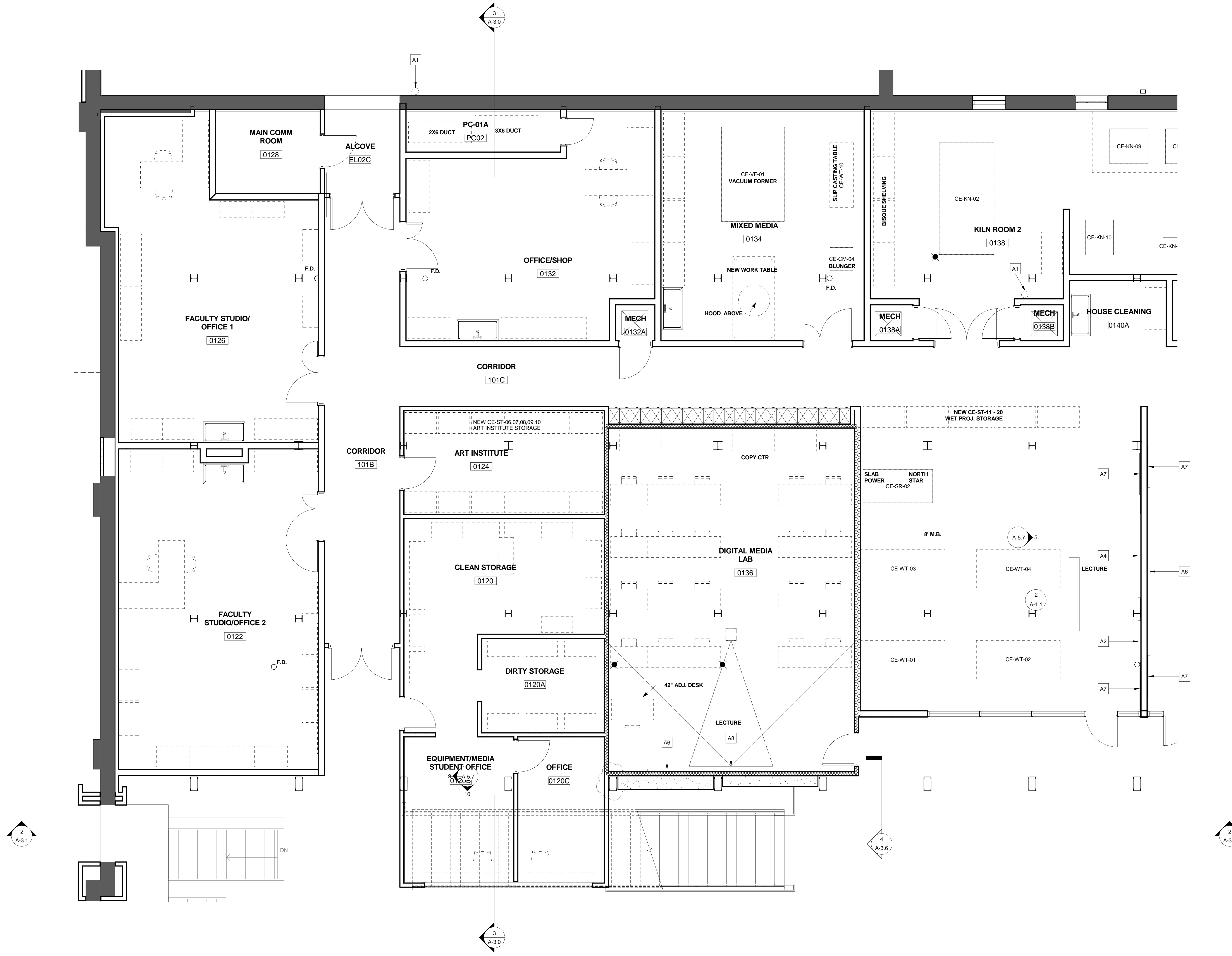
1 ENLARGED PLAN - CERAMICS A-5.24 1/4" = 1'-0"
