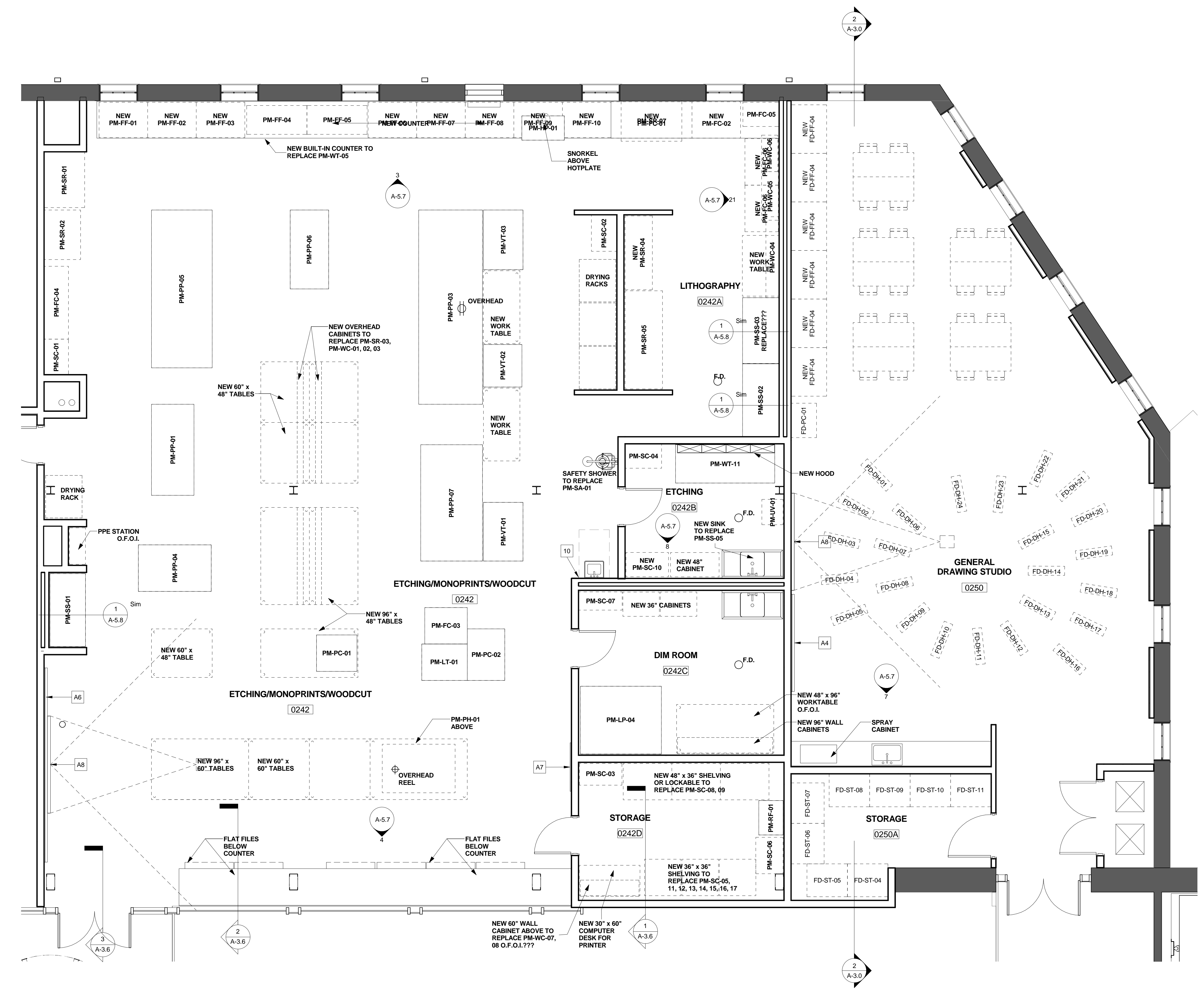
1 ENLARGED PLAN - PRINTMAKING A-5.28 1/4" = 1'-0"
