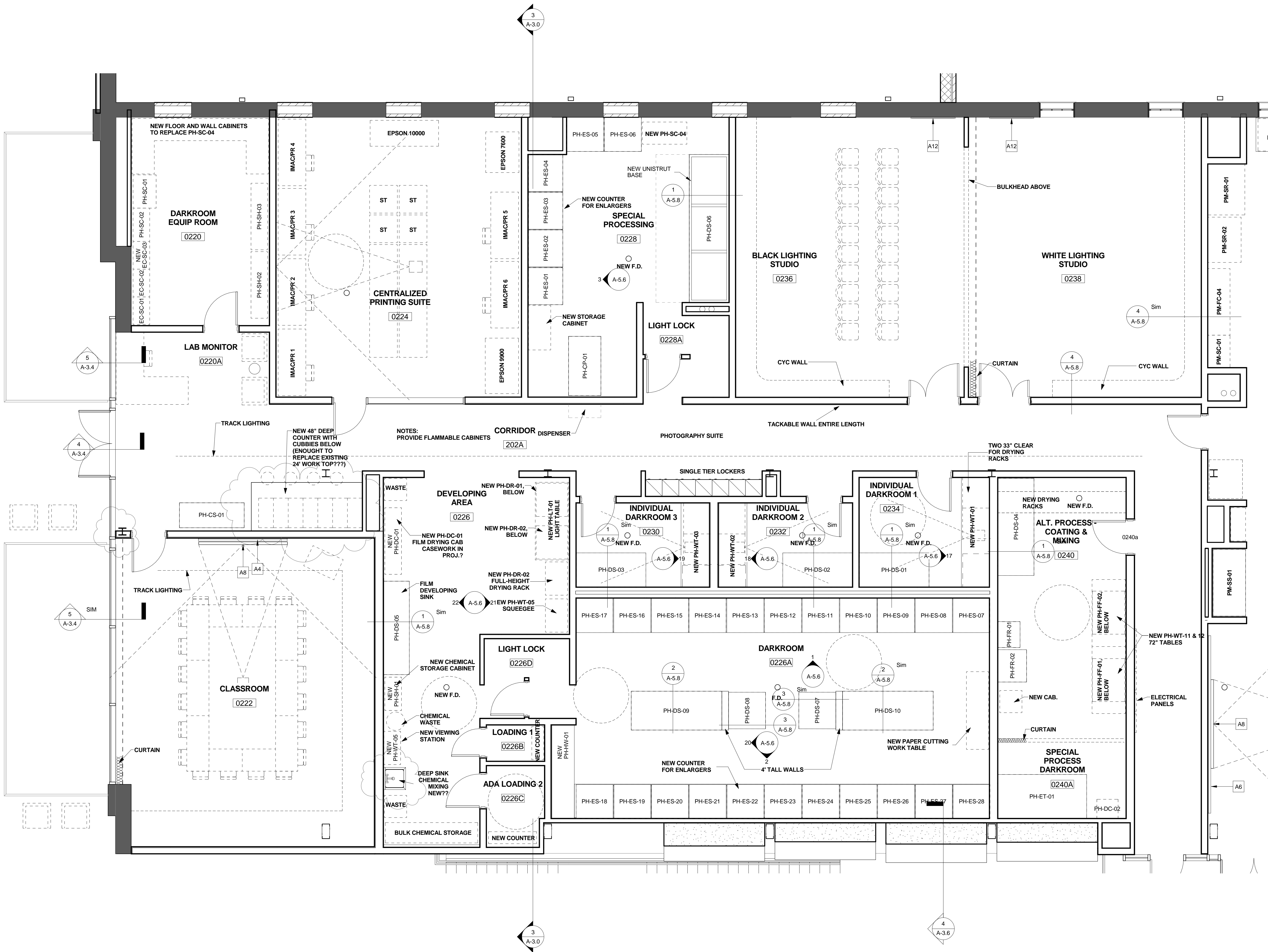
1 ENLARGED PLAN - PHOTOGRAPHY A-5.29/ 1/4" = 1'-0"
