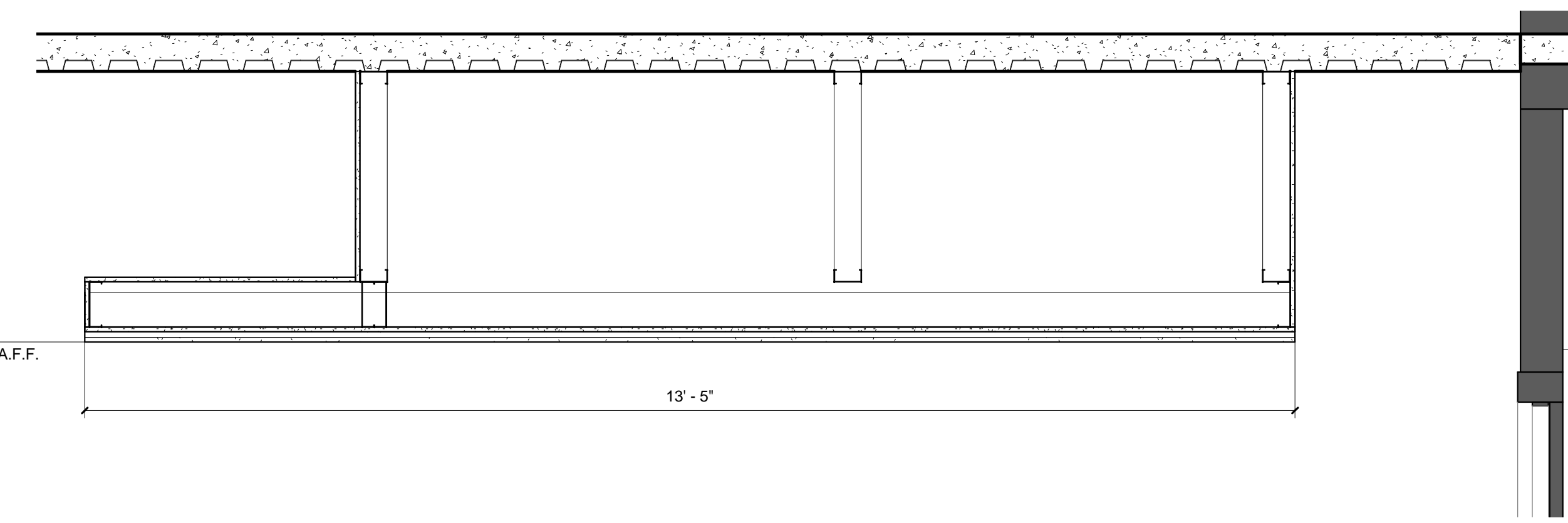
2 SOFFIT DETAIL A-6.0 / 3/4" = 1'-0"
