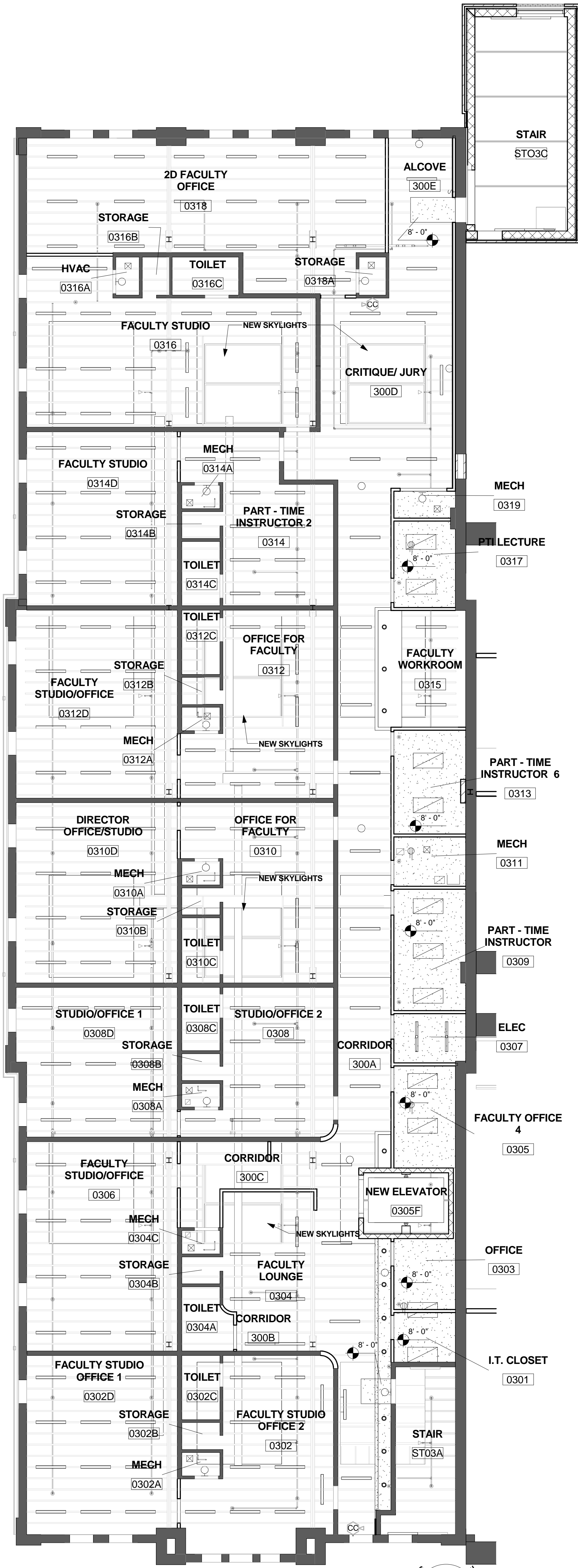
1 3RD LEVEL REFLECTED CEILING PLAN A-6.3 1/8" = 1'-0"
