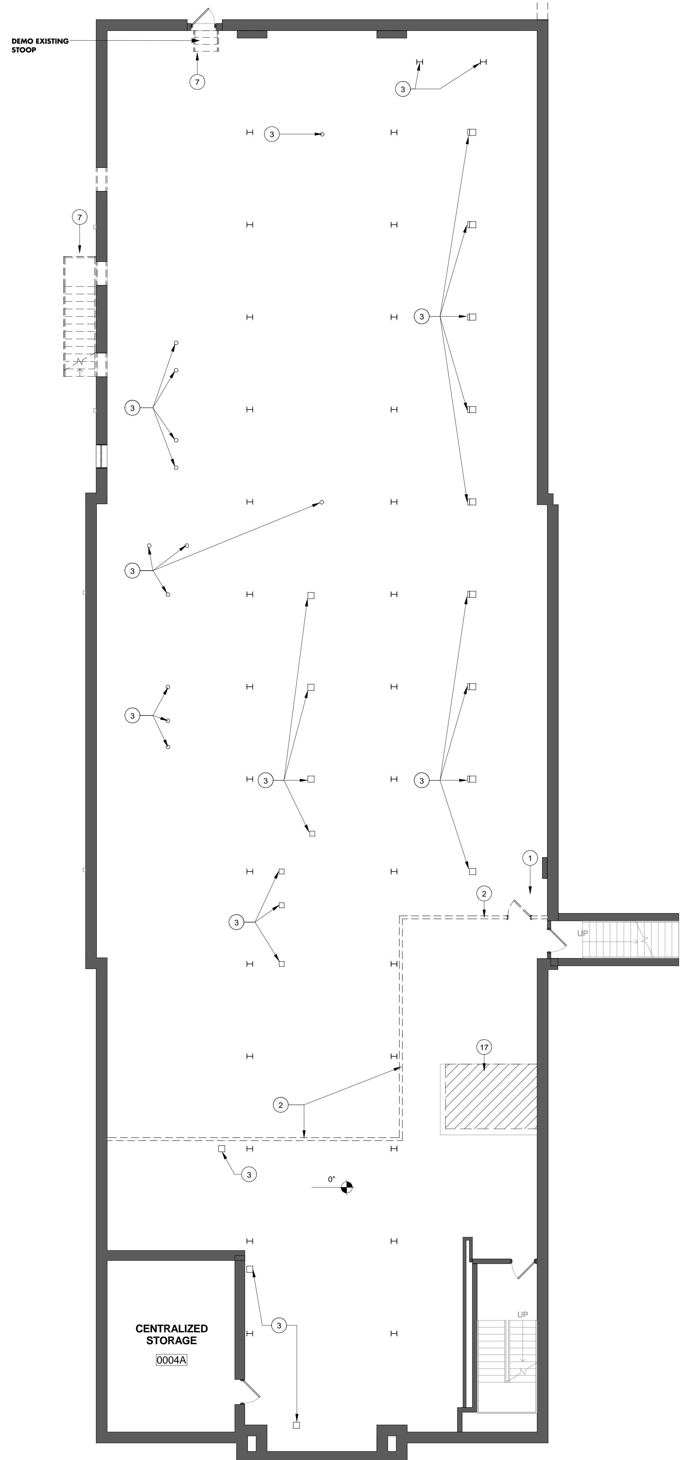
1 DEMOLITION PLAN - 0 BASEMENT D-1.0 1/8" = 1'-0"
