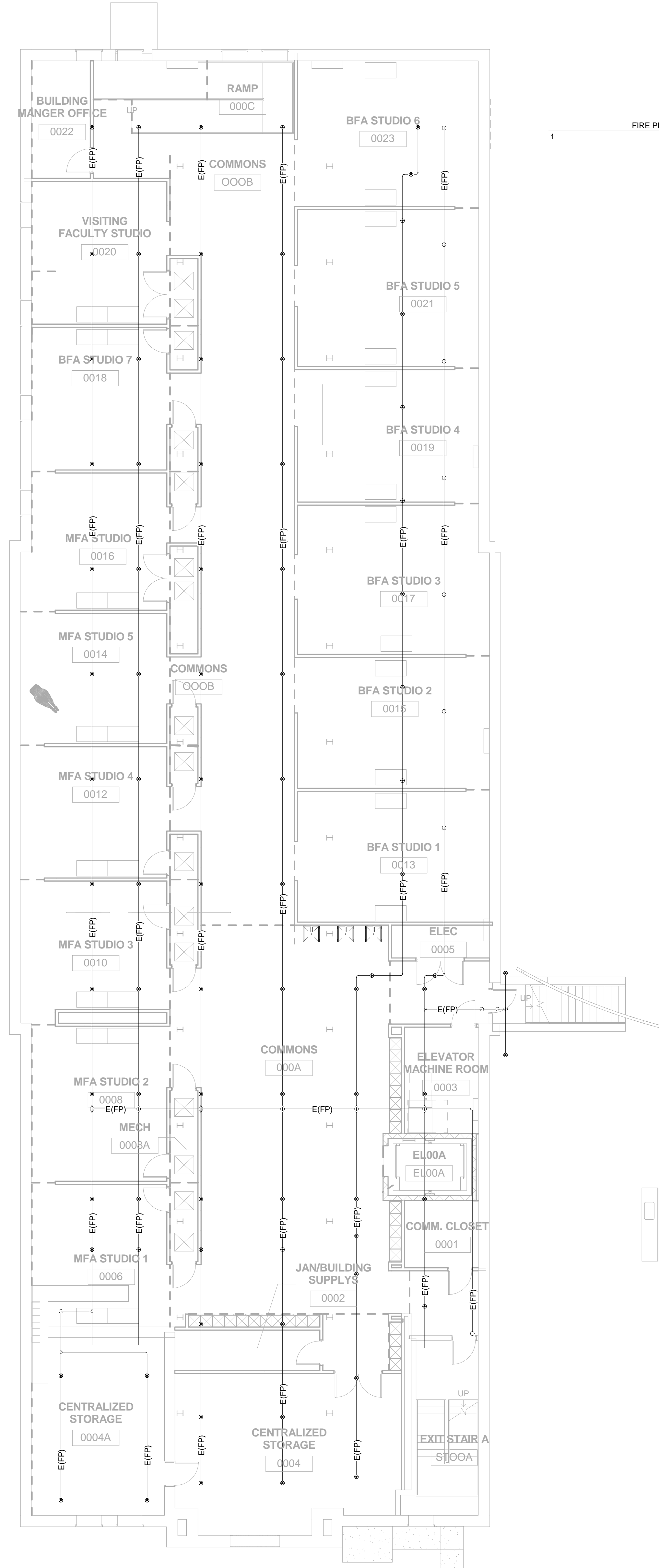
1 FIRE PROTECTION DESIGN BASEMENT PLAN 1/8" = 1'-0"
