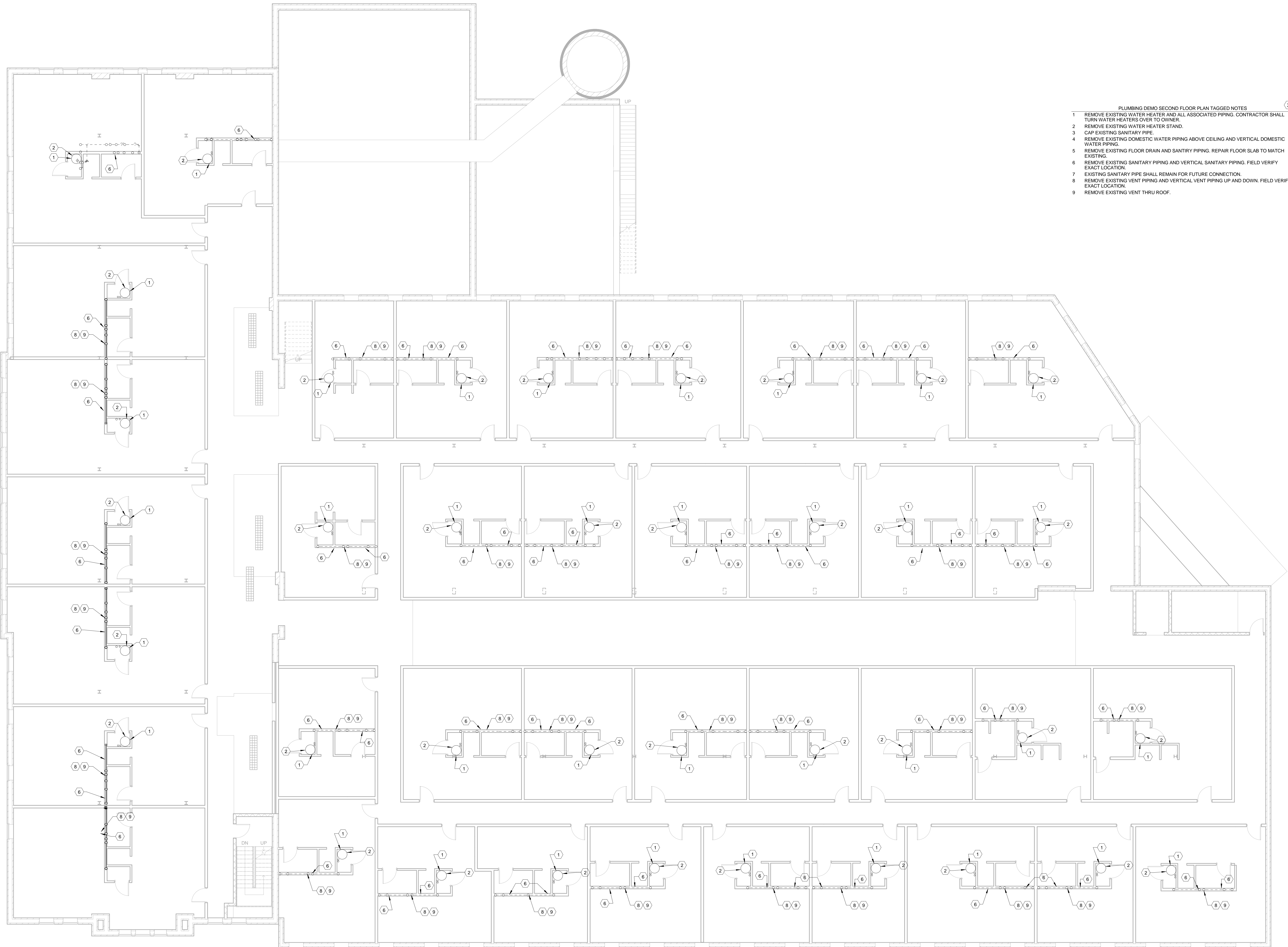
1 PLUMBING DEMO SECOND FLOOR PLAN 1/8" = 1'-0"
