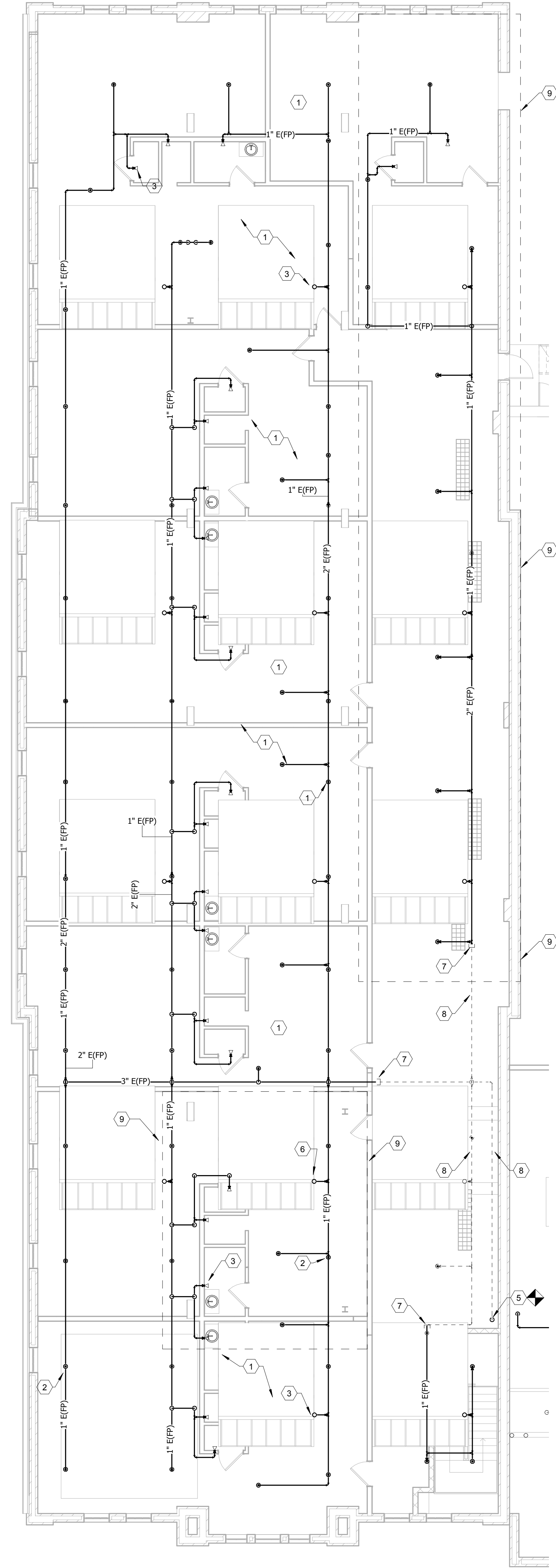
1 FIRE PROTECTION DEMO THIRD FLOOR PLAN 1/8" = 1'-0"
