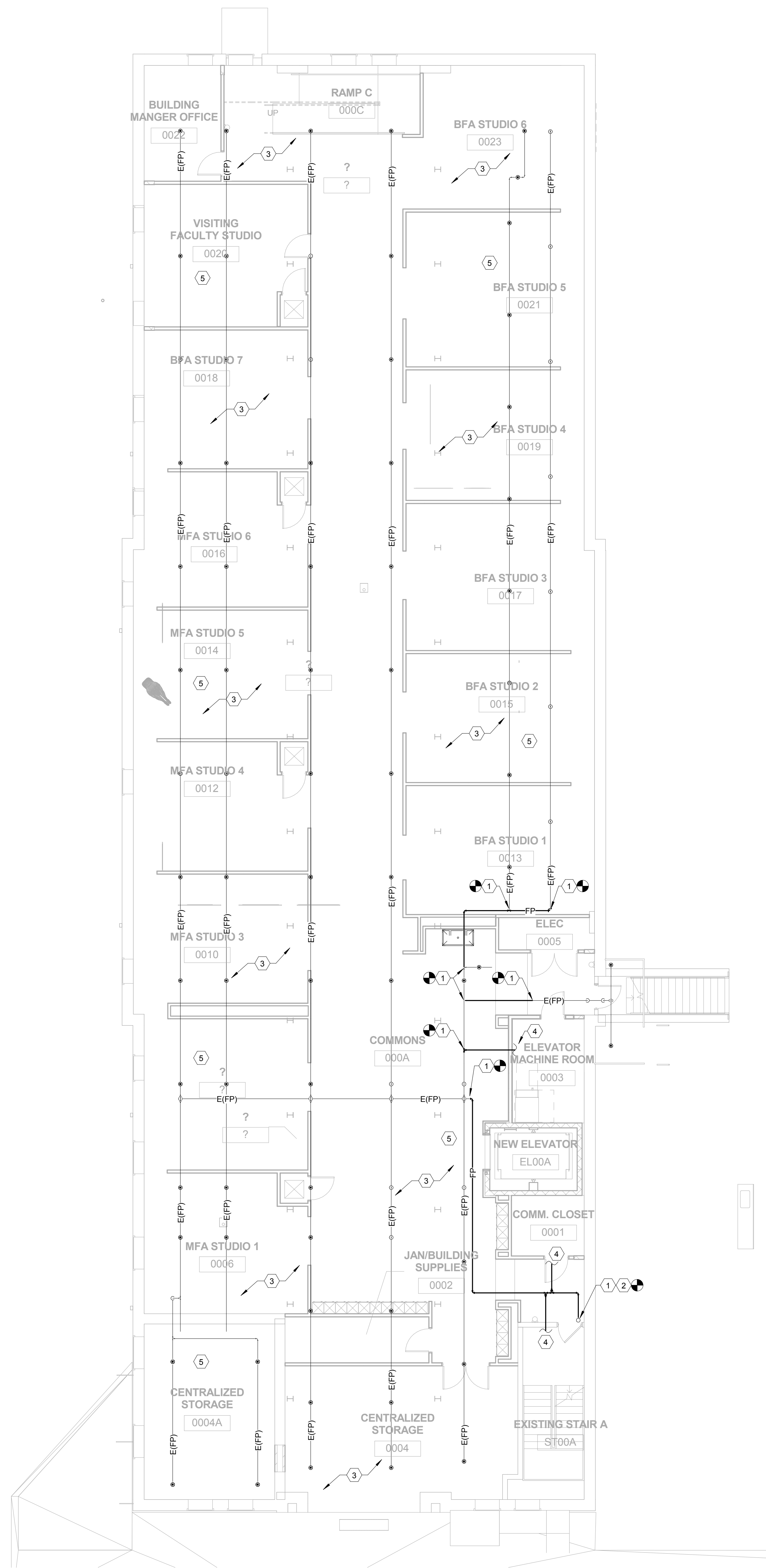
FIRE PROTECTION DESIGN BASEMENT PLAN - ALTERNATE 1/8" = 1'-0"
