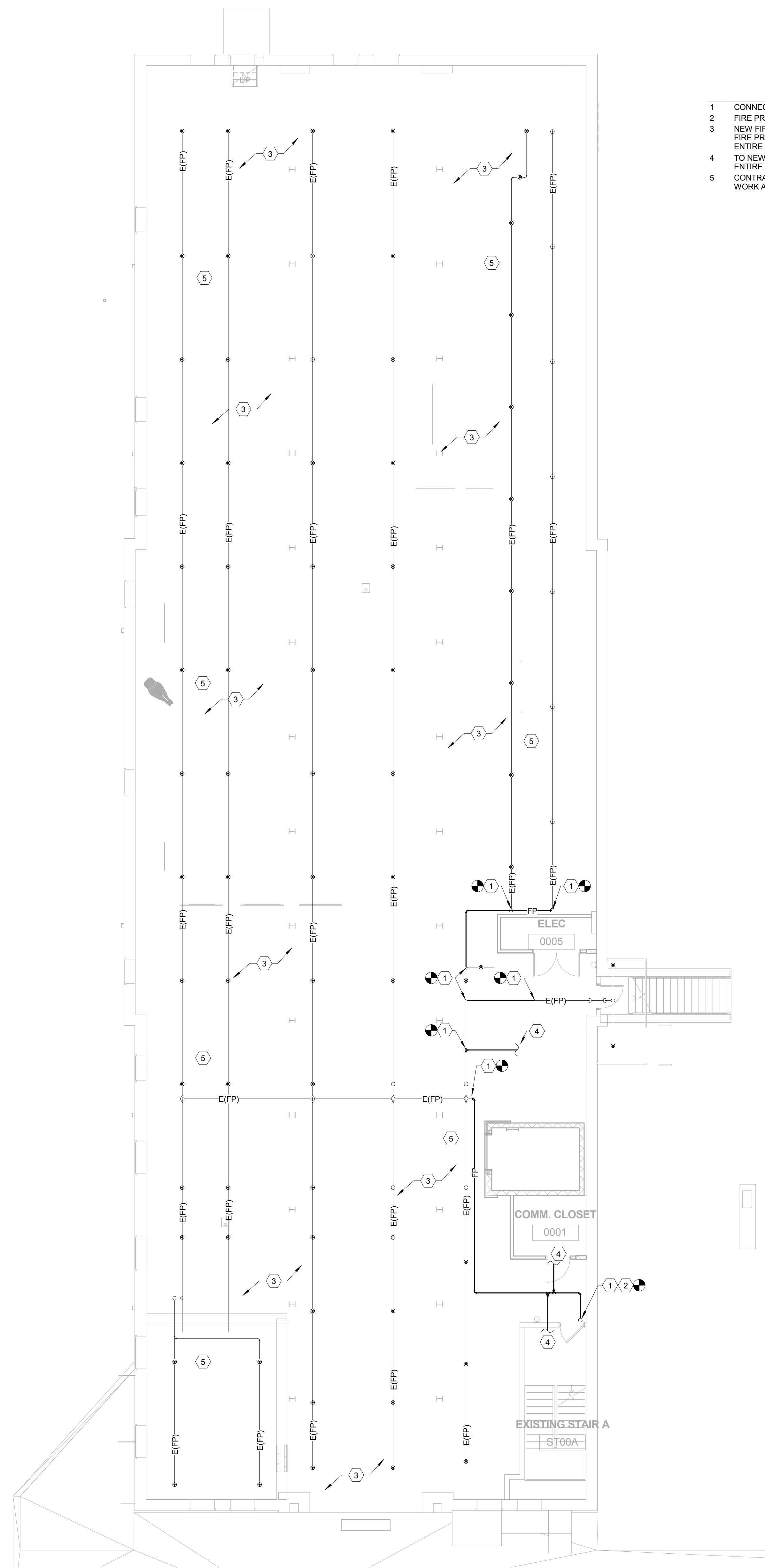
FIRE PROTECTION DESIGN BASEMENT PLAN - BASE BID 1/8" = 1'-0"
