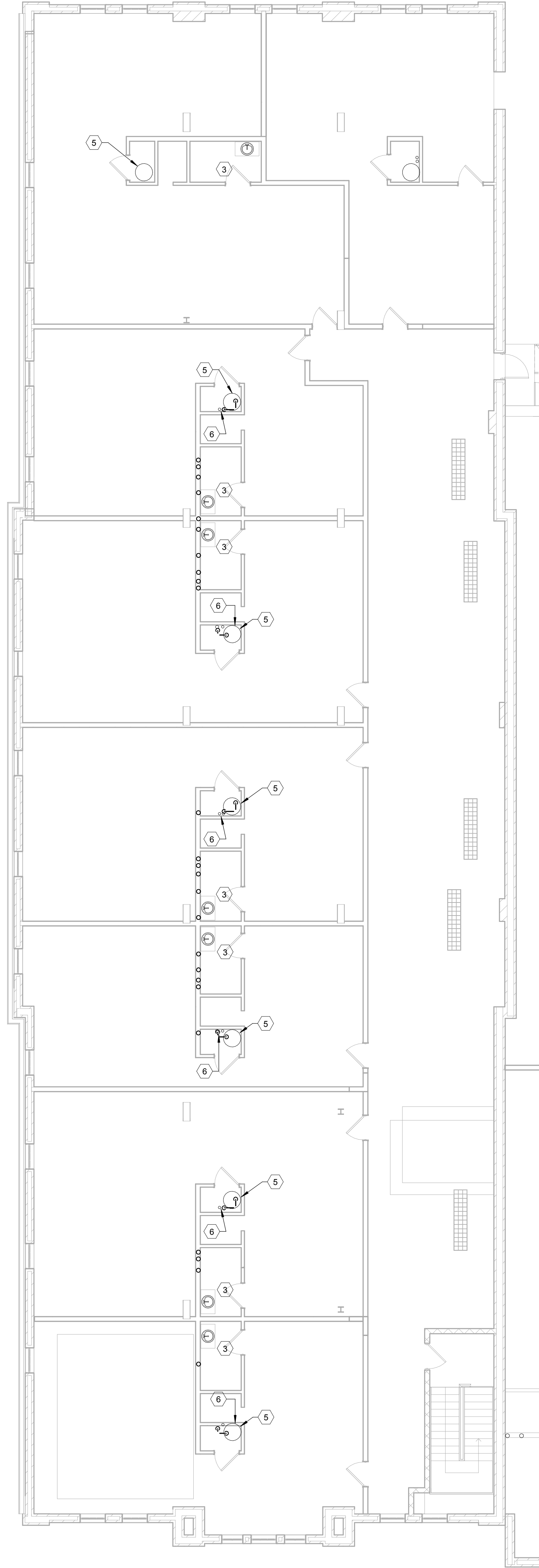
① PLUMBING DEMO THIRD FLOOR PLAN - BASE BID 1/8" = 1'-0"
