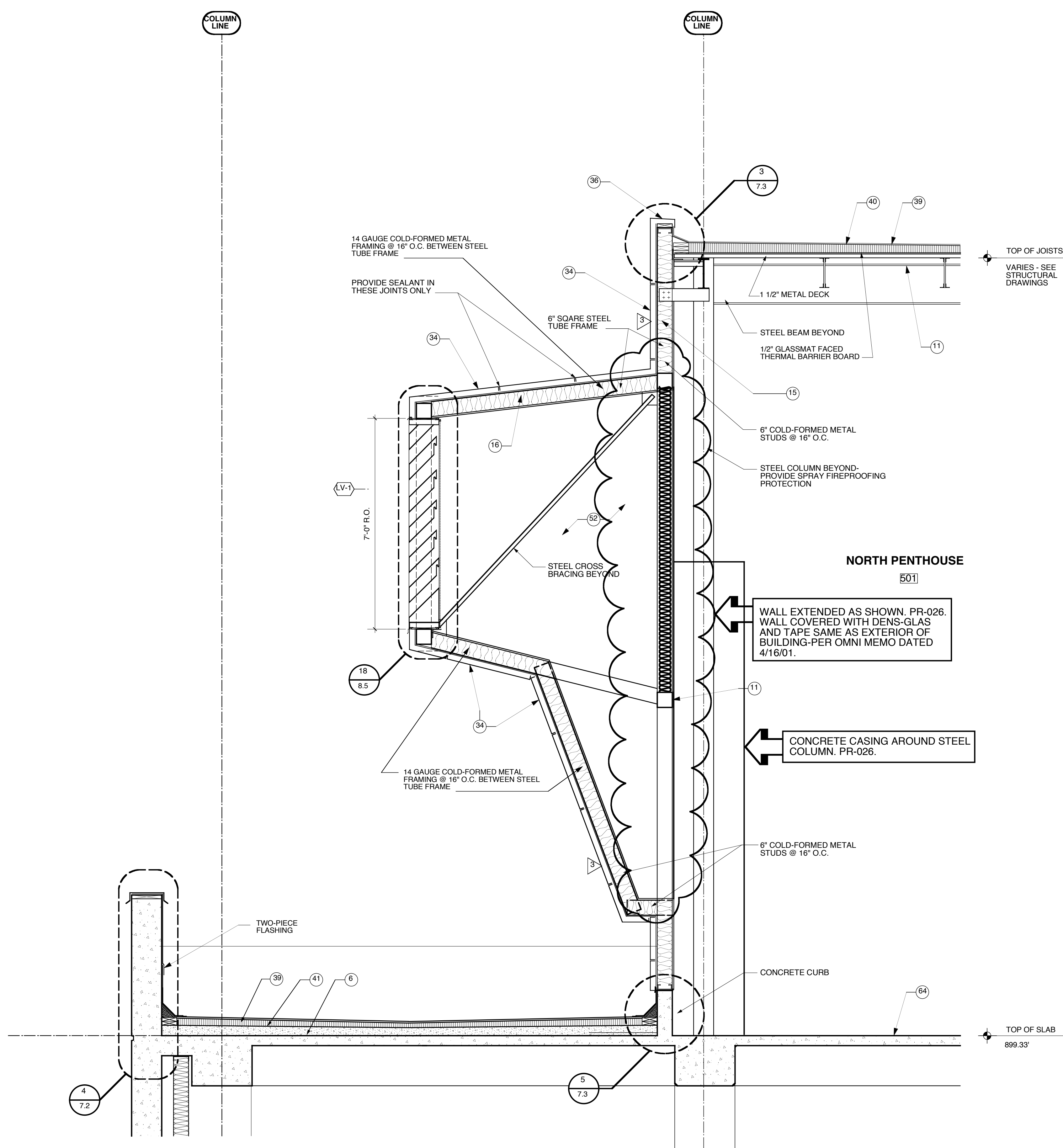
13 WALL SECTION @ ENDWALL OF NORTH PENTHOUSE
