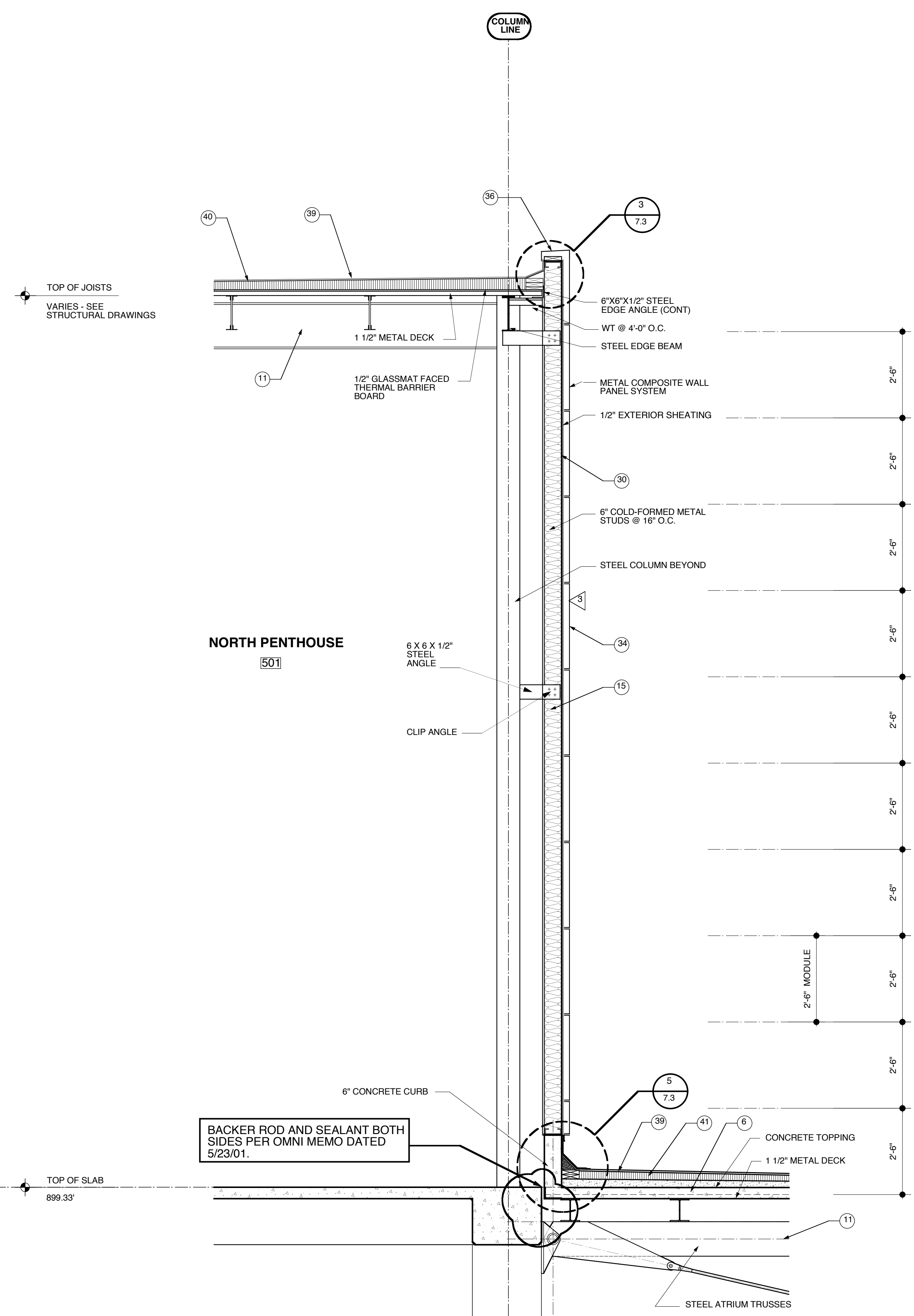
11 WALL SECTION @ ATRIUM OF NORTH PENTHOUSE
