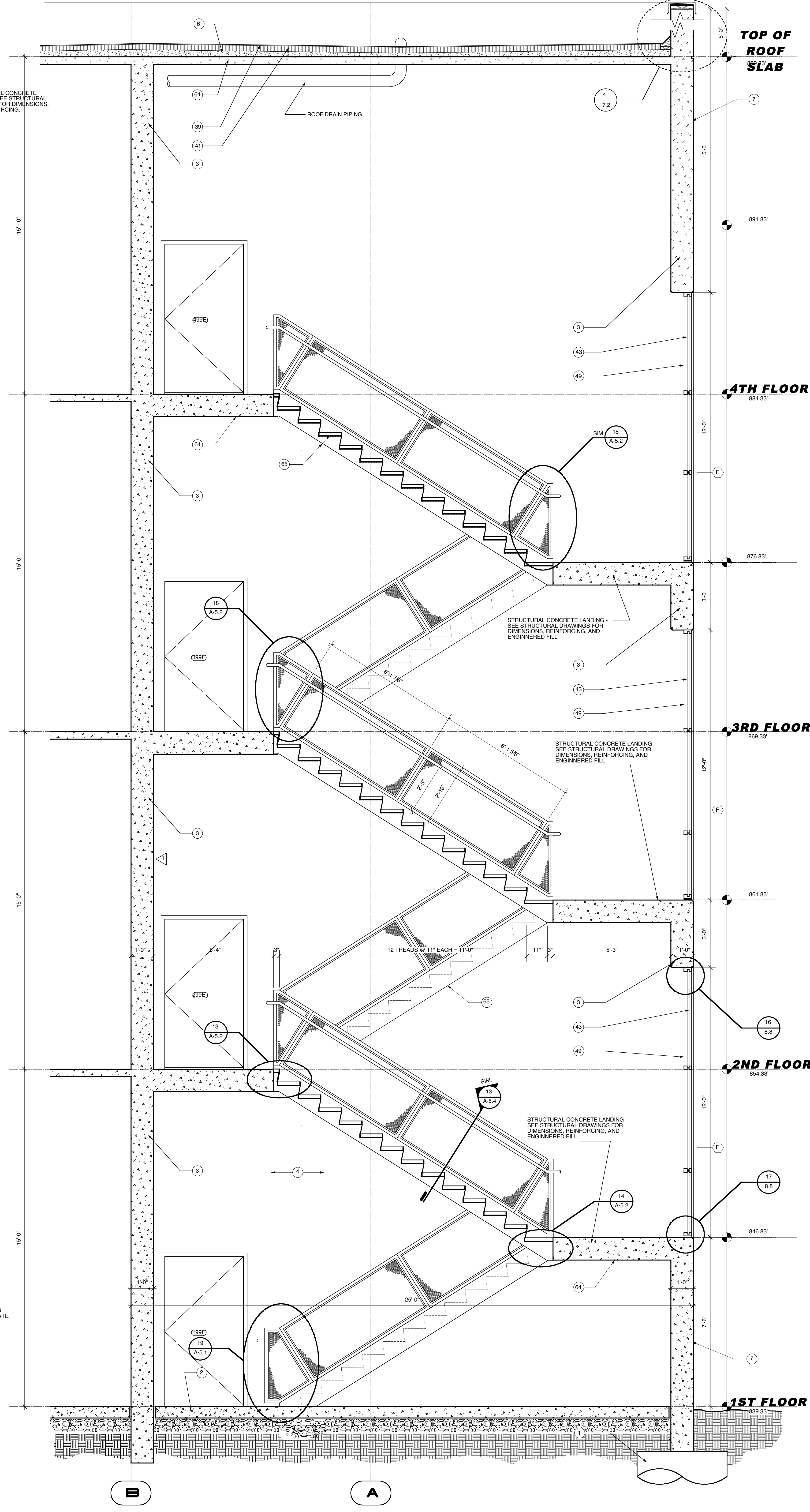
14 STAIR "A" SECTION 1/2" = 1'-0" NOTE: REF. TO SHEET A-4.12 FOR KEY NOTES
