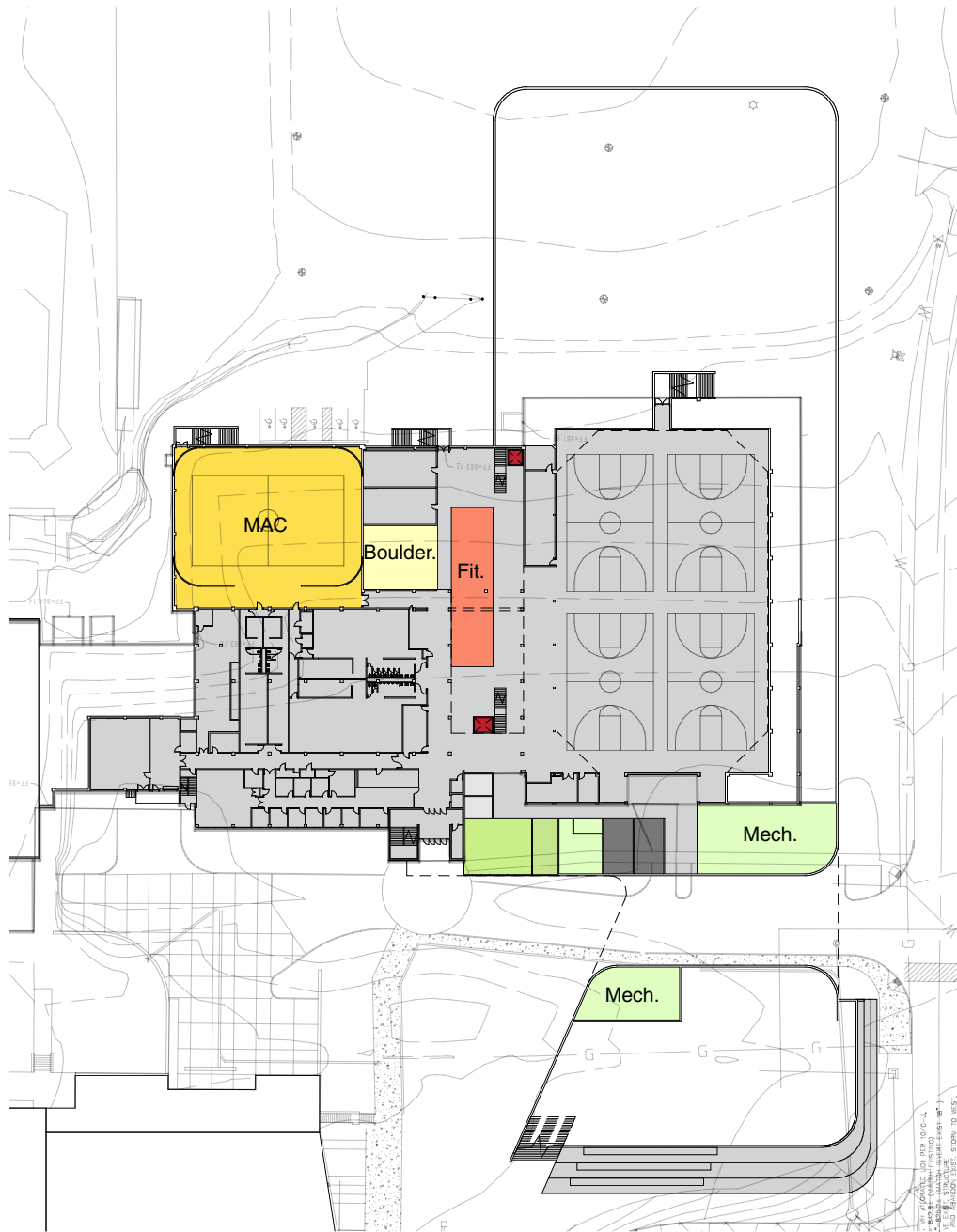
Scheme B First Floor Plan
