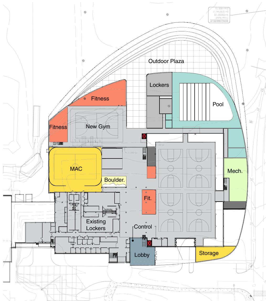
Scheme A First Floor Plan
