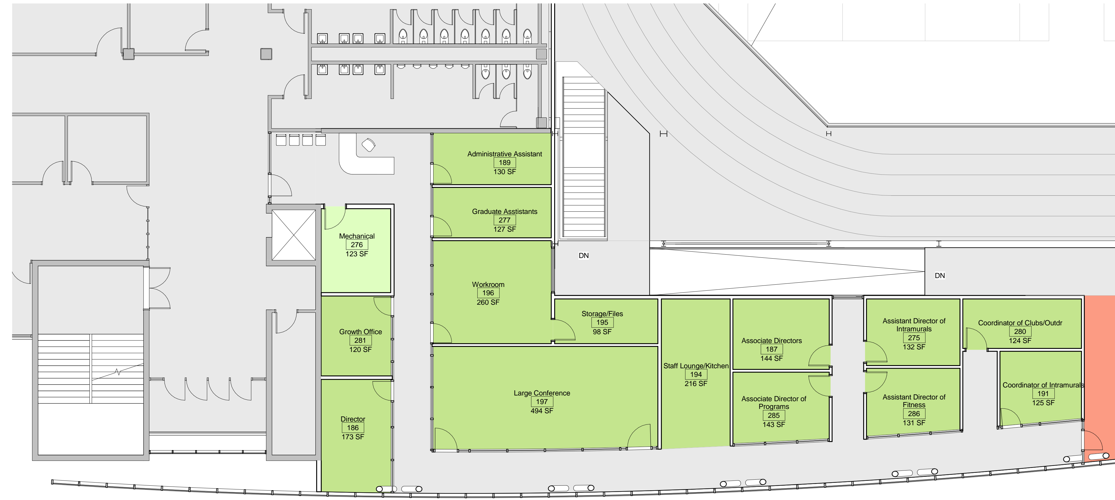
2 ENLARGED PLAN @ ADMINISTRATION SUITE 1/8" = 1'-0"
