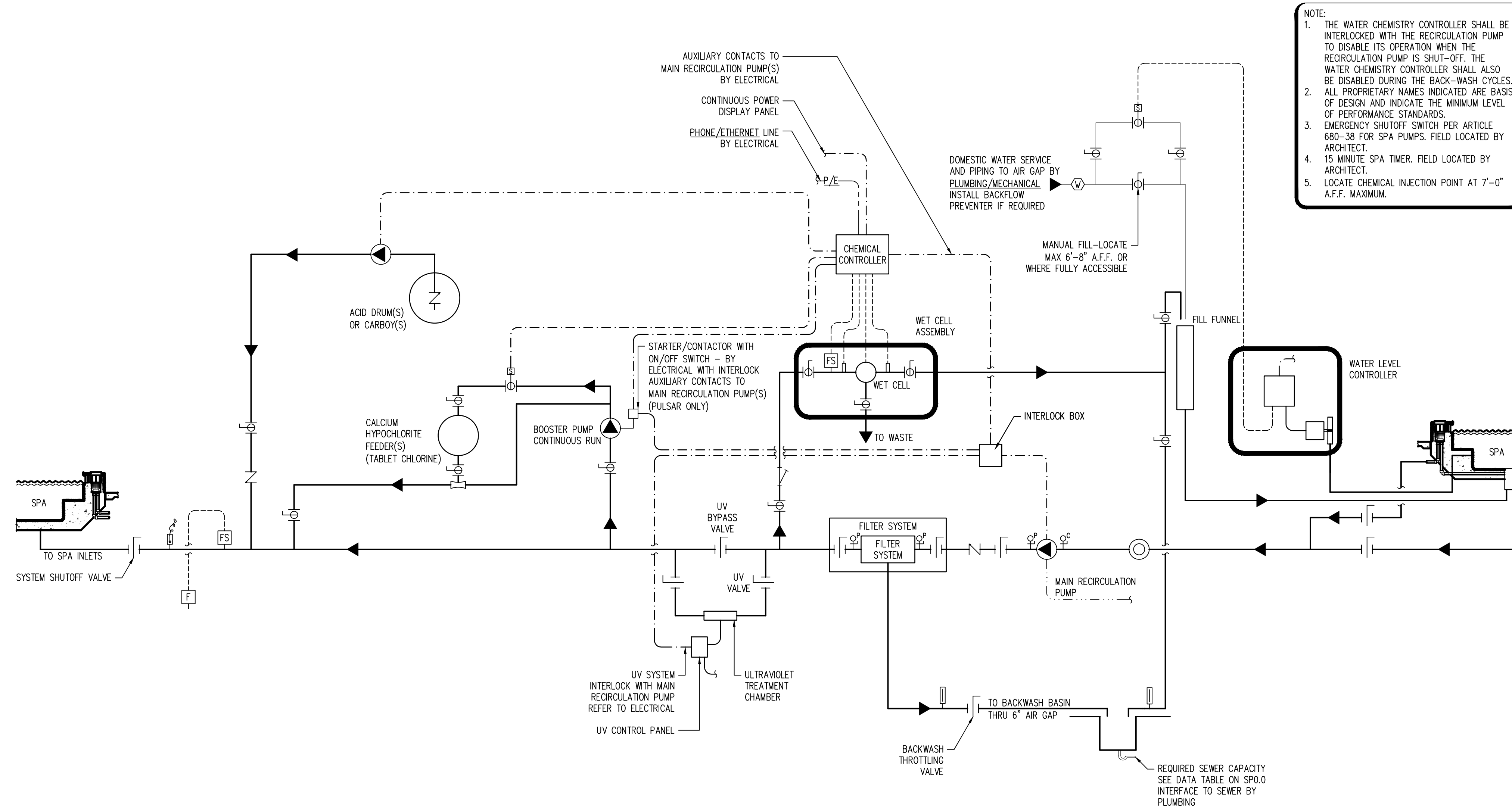
2 SPA SYSTEMS SCHEMATIC SP-6.0 NTS 07/09/12
