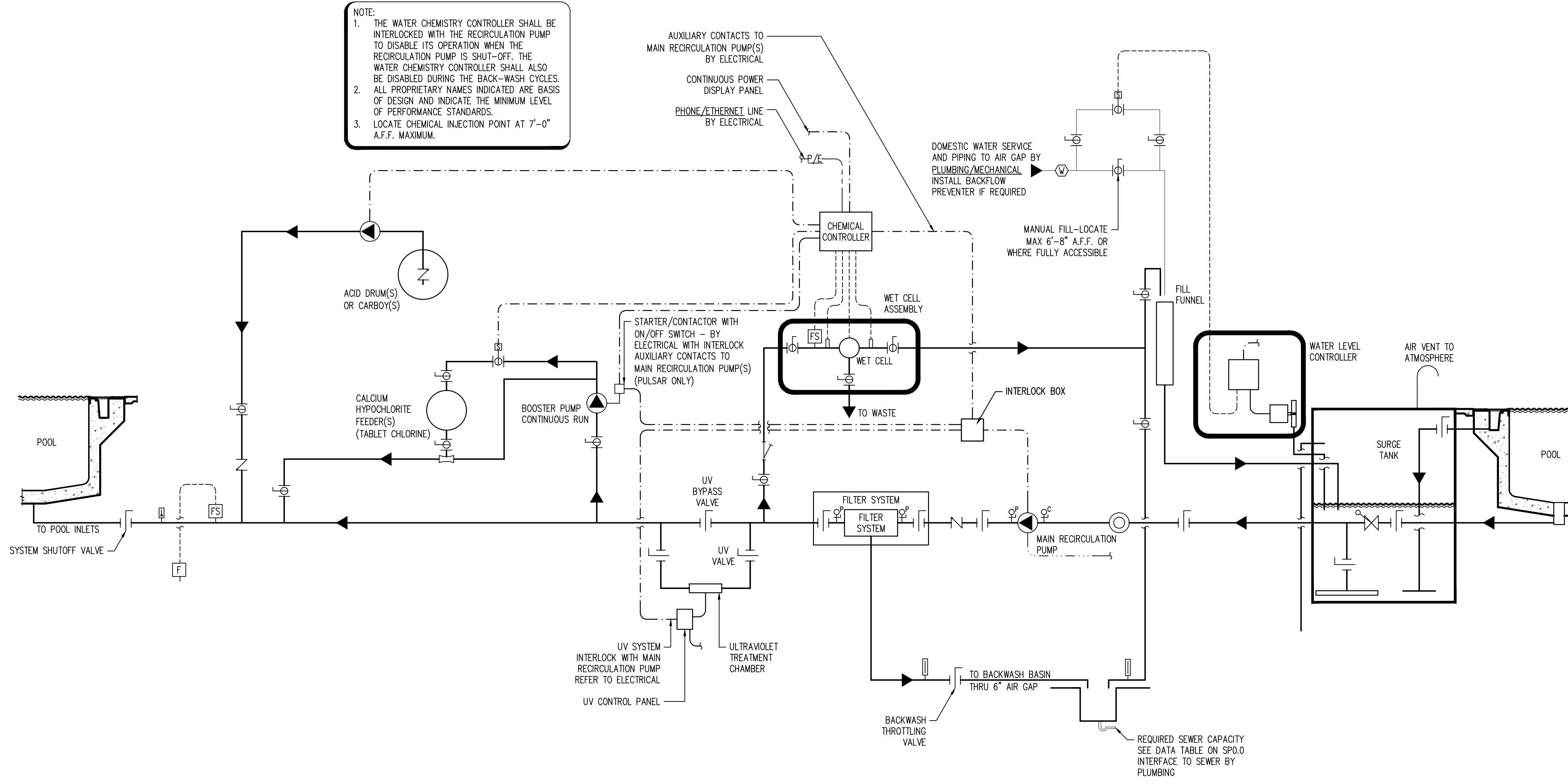
1 POOL SYSTEMS SCHEMATIC SP-6.0 NTS 07/09/12
