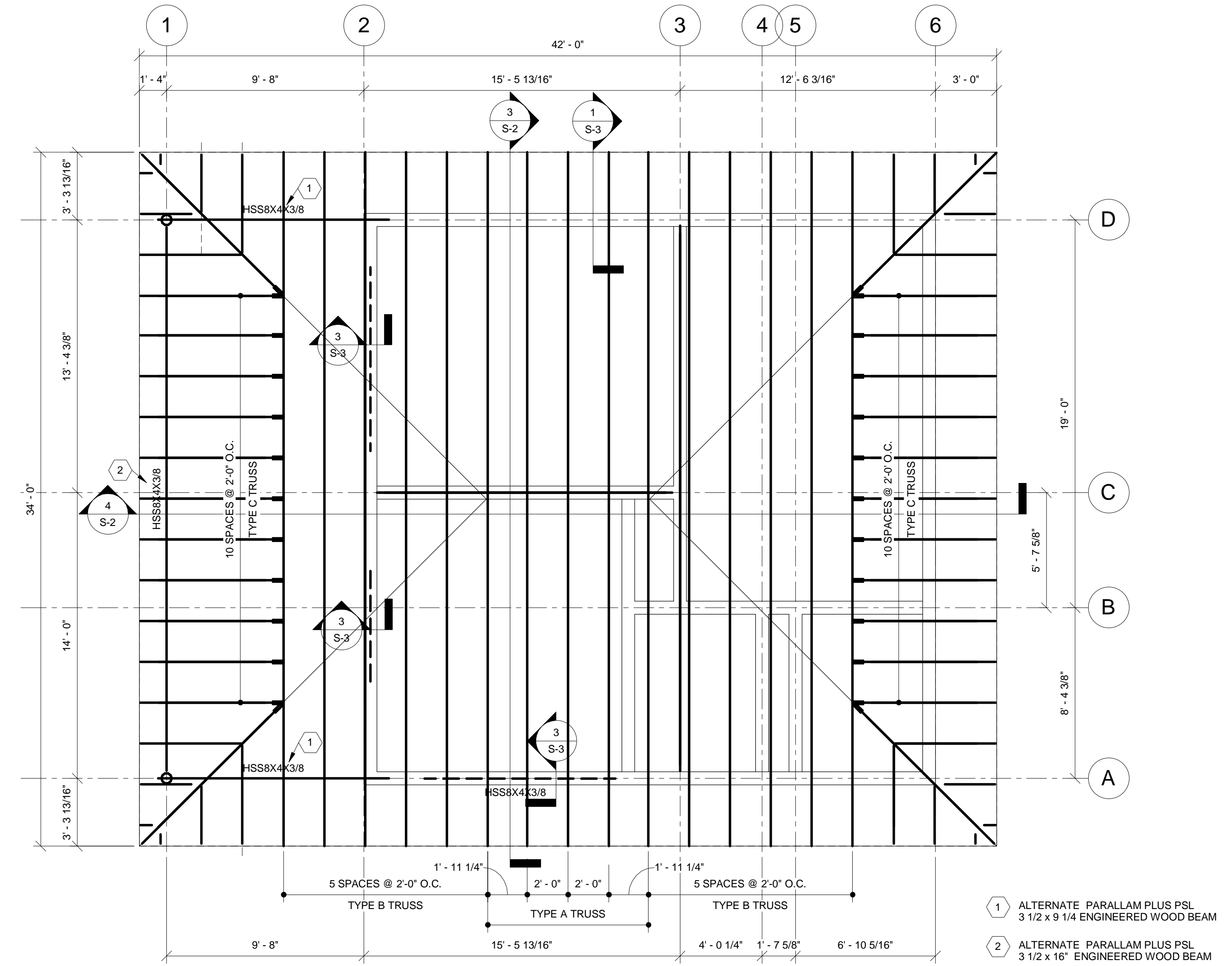
2 PLAN DETAIL S-2 1/4" = 1'-0"
