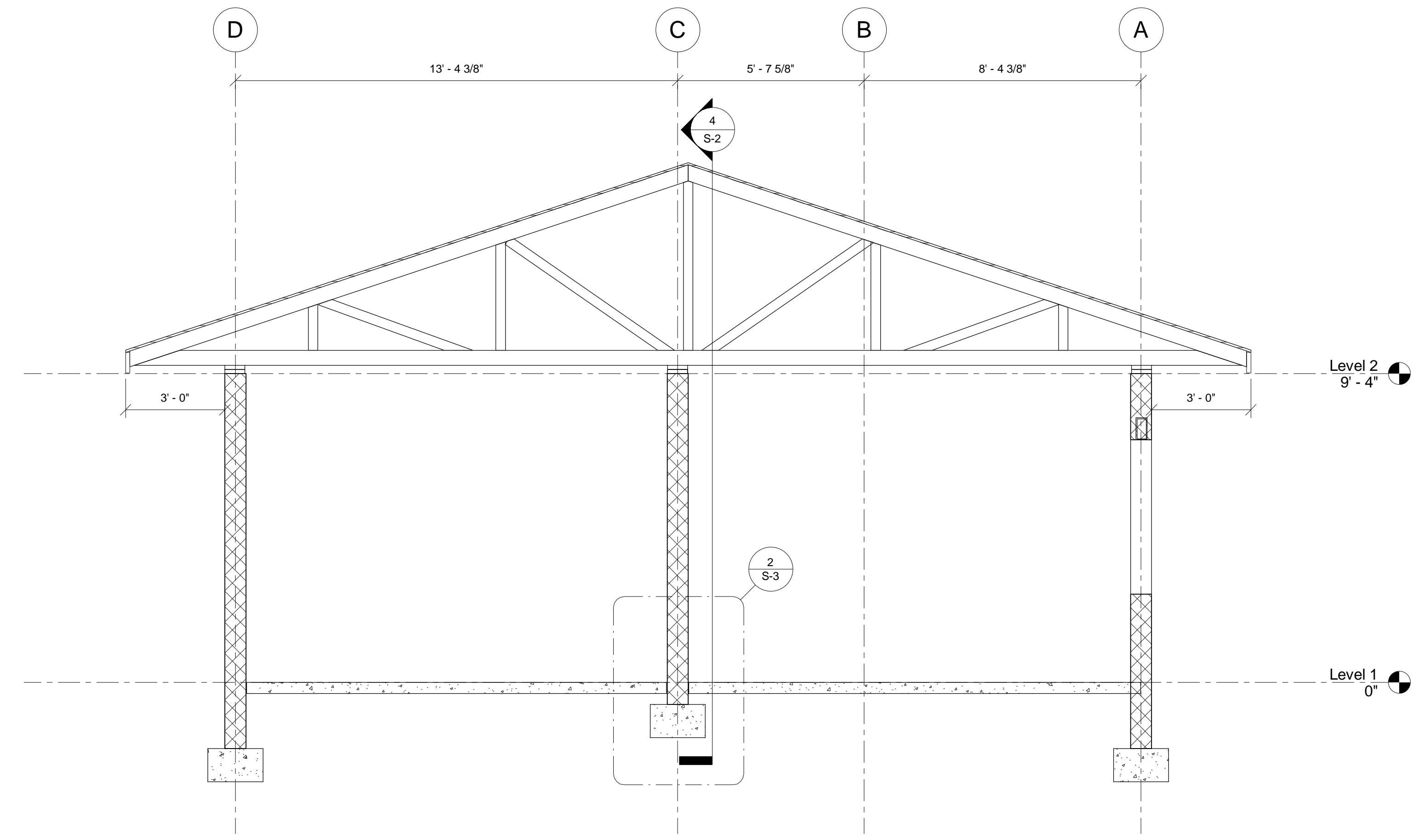
3 SECTION S-2 3/8" = 1'-0"
