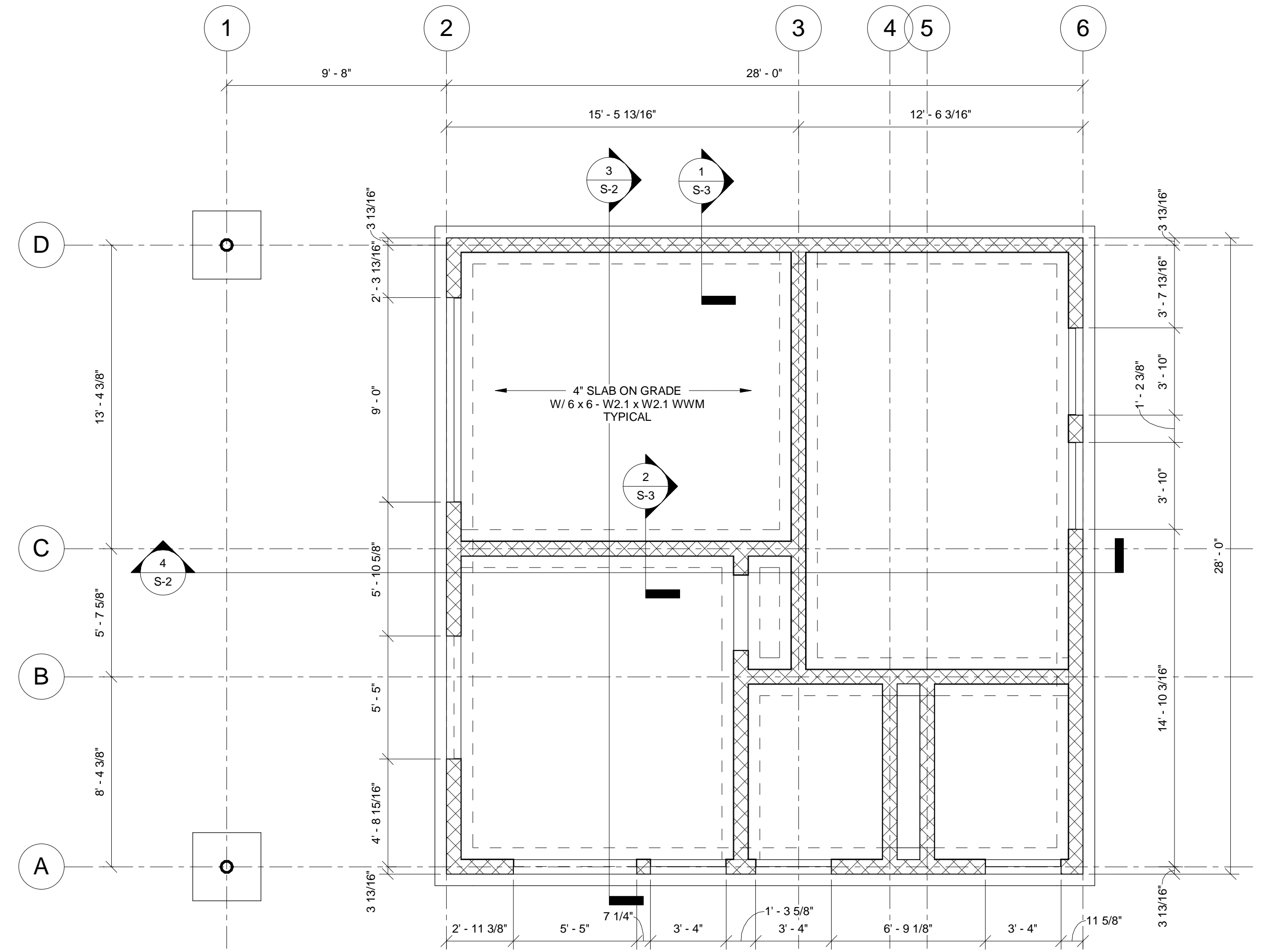
1 PLAN DETAIL S-2 1/4" = 1'-0"
