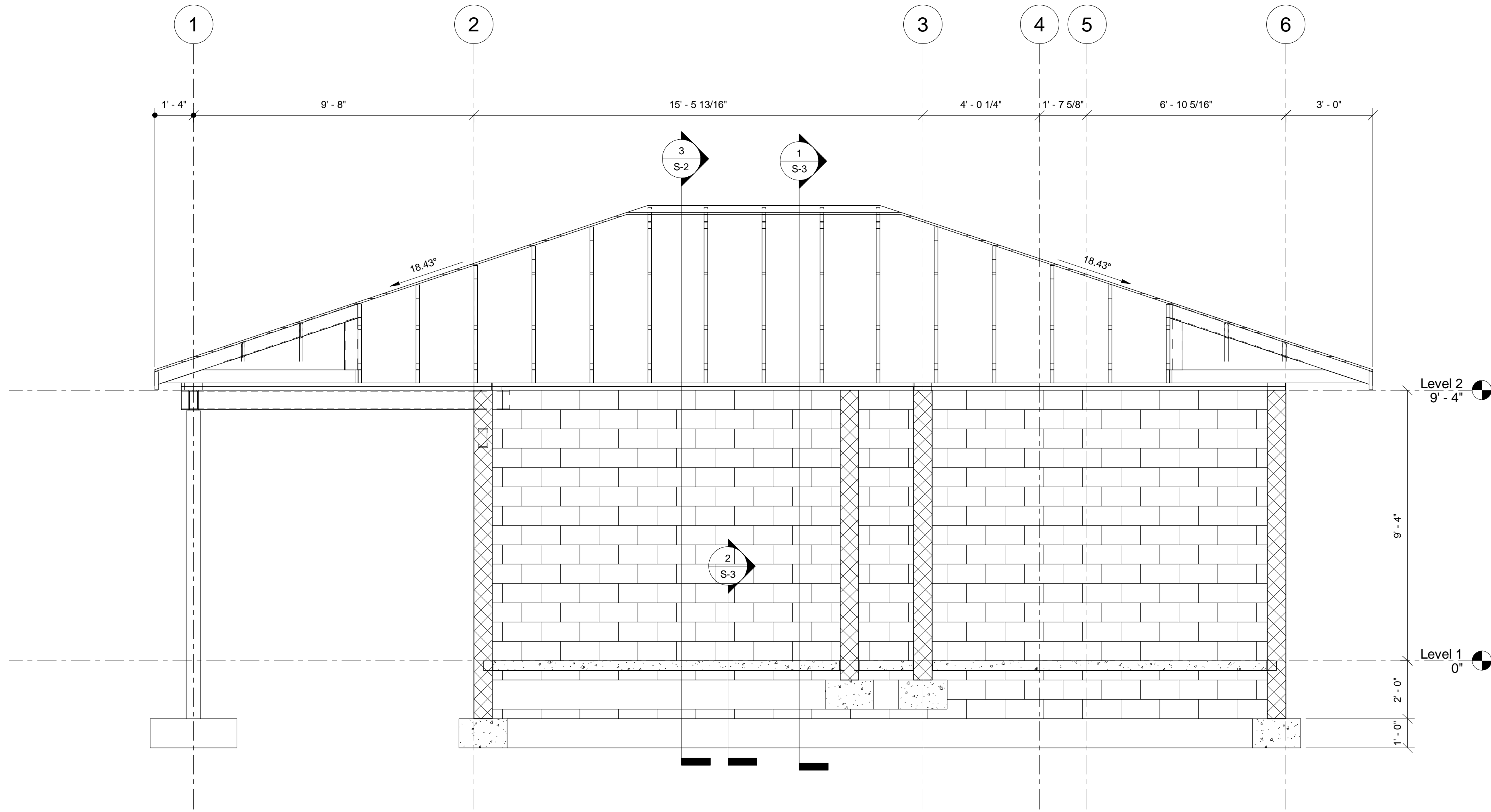
4 SECTION S-2 3/8" = 1'-0"
