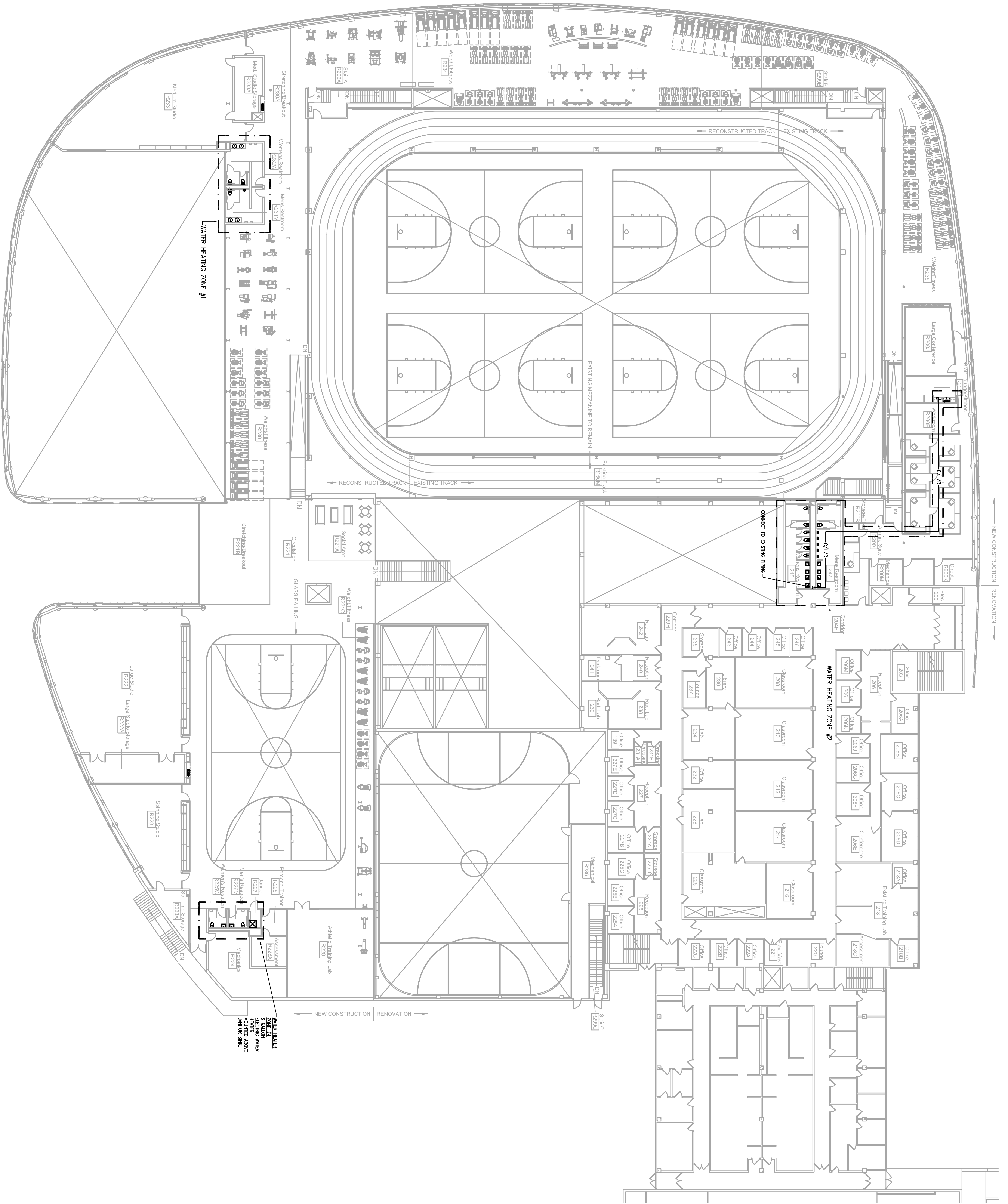
SECOND FLOOR PLAN - PLUMBING
