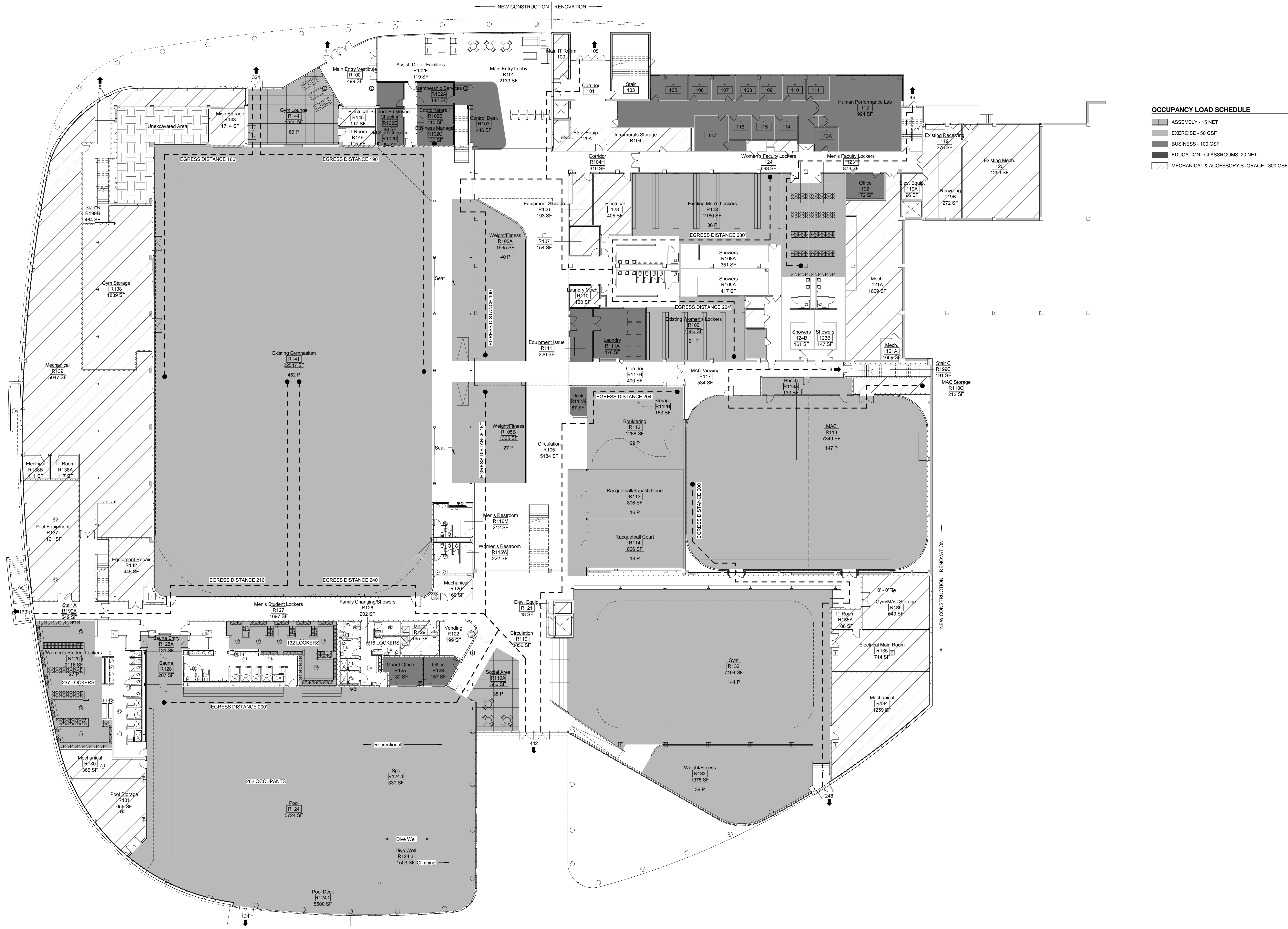
1 LEVEL 01 - CODE REVIEW 1/16" = 1'-0"
